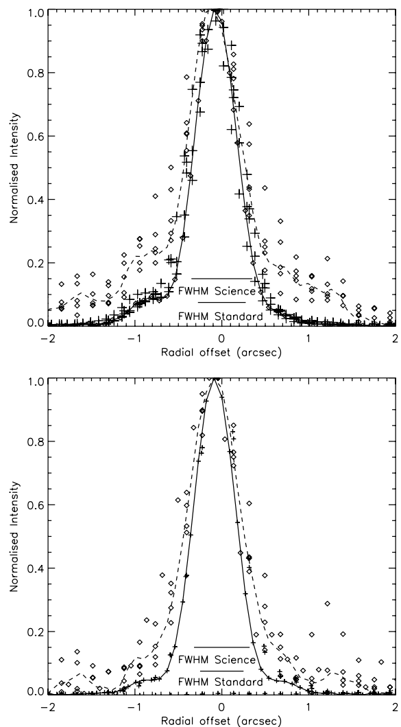
Figure 2. The profile of the line cuts through the total images at 80^\circ east of north (top) and 170^\circ east of north (bottom). The median FWHM measurements taken over all subintegrations from Gaussian fits to the profiles at the two angles are indicated for reference. The averaged profiles from all the line cuts for both HD 191089 and the standard star are also shown. The profile for HD 191089 (dashed line) at 80^\circ is much broader in the wings than that of the standard star (solid line). There is also some evidence of a less pronounced extension at 170^\circ as seen in the lower image. Note that multiple intensity profiles for the science target (diamonds) and the standard (crosses) are shown here. These are taken for each group as indicated in Table 1.
