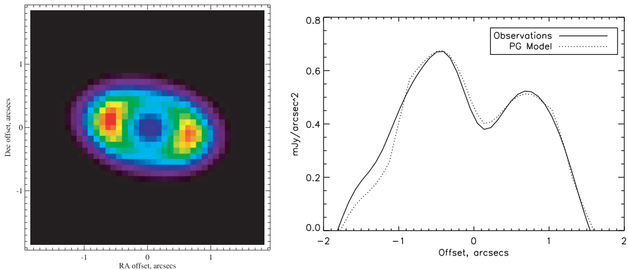
Figure 5. The best-fitting disc from the pericentre glow model which is scaled and shown in the same way as the HD 191089 residuals (Fig. 1) for comparison. The disc parameters are the same as those for the best-fitting axisymmetric disc shown in Fig. 3 (28–90 au, i = 35^\circ , \Sigma \propto r^\gamma ). Right: linecut through the observed and model images at a PA of 80^\circ (observed: solid line; model: dotted line).
