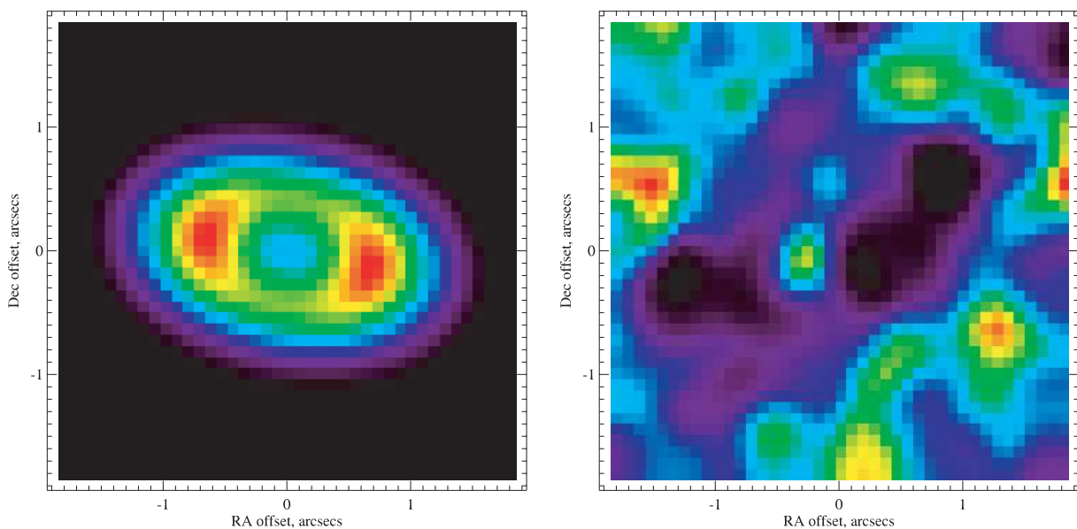
Figure 3. The best fitting axisymmetric disc model for the 18\text{-}\mu\text{m} emission (see Section 4.1). The model residual image (left) can be compared directly with the observed residuals (Fig. 1, right). The difference between the observed residuals and the model residuals (right) indicates an over subtraction near the ansae and a slight under subtraction at the peak. See section 5.1 for details.
