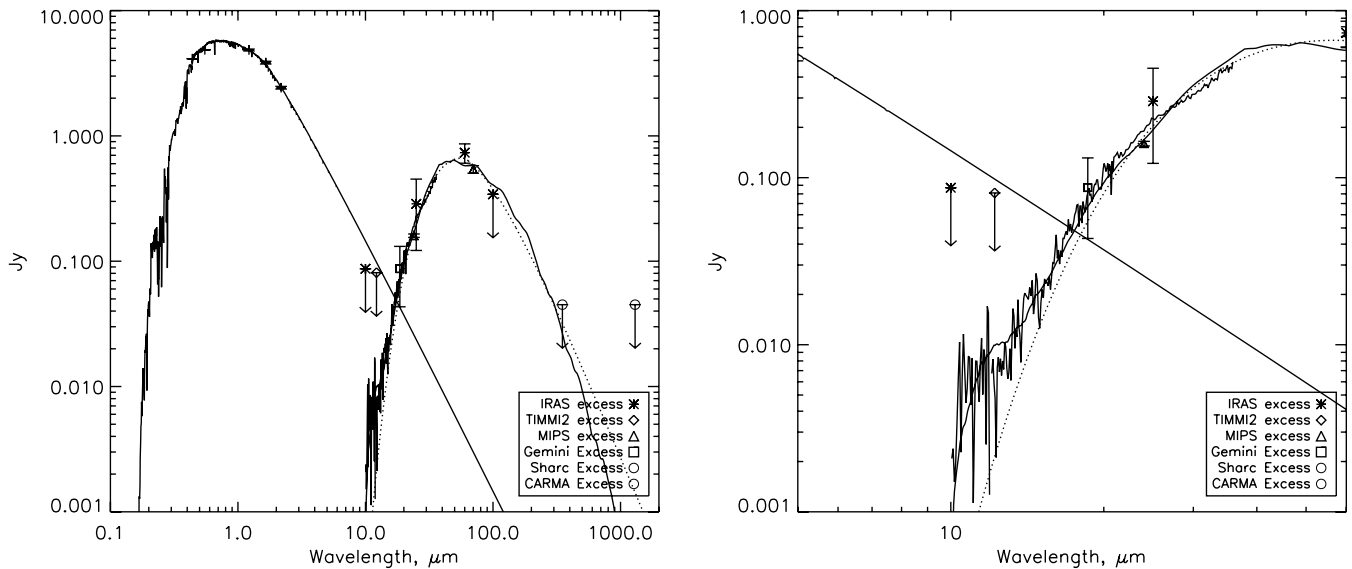
Figure 4. SED of HD 191089. The photosphere of HD 191089 is fitted with a Kurucz model profile ( M_{\text{star}} = 1.4 M_{\odot} , L_{\text{star}} = 3.2 L_{\odot} , T_{\text{star}} = 6440 K) scaled to the 2MASS K -band flux and shown with a solid line. Observations at >5 \mu\text{m} are shown after the subtraction of the photospheric contributions: the IRS spectrum of Chen et al. 2006 (solid line from 5 to 30 \mu\text{m} ), MIPS fluxes (Carpenter et al. 2009) (triangles) and IRAS colour-corrected excesses (asterisks) and Gemini TRCs fluxes in 0.5 arcsec radius aperture (square), and submm/mm upper limits (crosses) from SHARC and CARMA. The excess measurements are first fitted with a 99 K modified blackbody (dashed line), for comparison to a realistic grain fit (solid line) described in Section 4.2.
