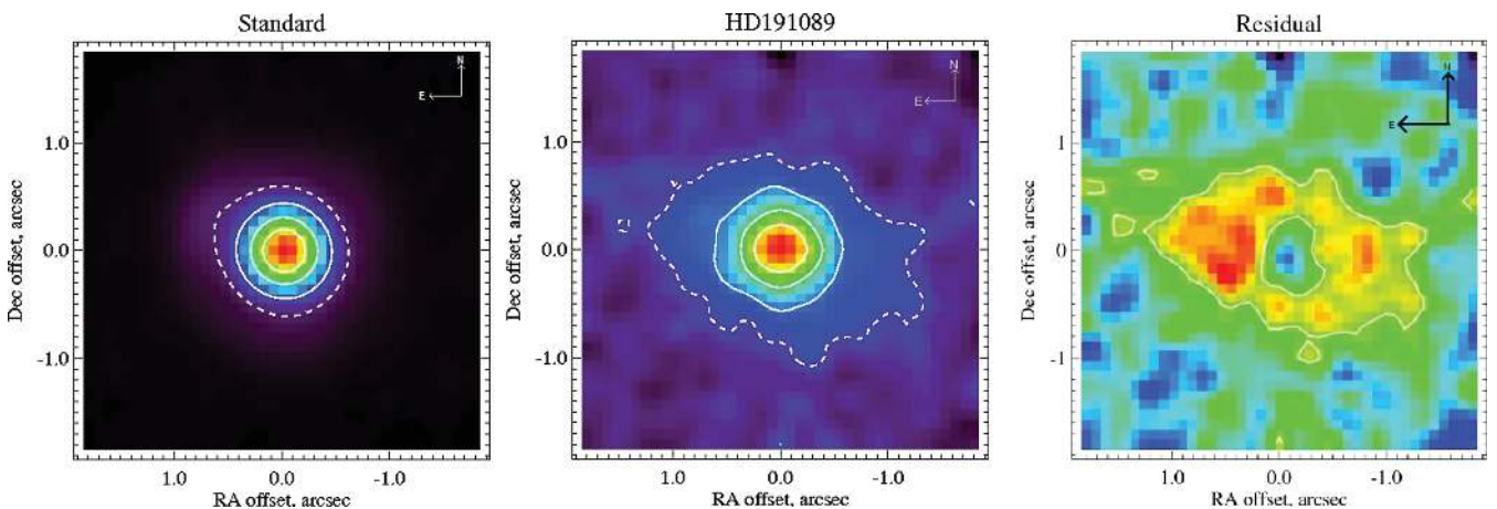
Figure 1. Left to right: the final co-added images of the standard star (left) and HD 191089 (centre) and a residual emission image shown after subtracting an azimuthally symmetric PSF created from the standard star image scaled to the expected photospheric emission from HD 191089 ( 44 \text{ mJy} ) from the science image (centre). Note that the distinct ellipticity seen in the image of HD 191089 is not seen in the standard star. Contours on the left and central plots are at 25, 50 and 75 per cent of the peak (solid lines) and 10 per cent of the peak (dashed line). The contours on the residual emission image are at 25, 50 and 75 per cent of the peak. Orientation of the images is north up, east left. The peak value for HD 191089 in Qa is 344 \text{ mJy arcsec}^{-2} and the peak value for the standard is 27\,648 \text{ mJy arcsec}^{-2} . The peak value for the residuals is 55 \text{ mJy arcsec}^{-2} . The residual image has been smoothed by convolving with a Gaussian with a width of 4 pixels. The colour scale is linear from 0 to the maximum pixel value in each image.
