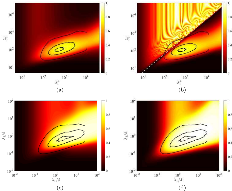
Figure 1: Energy contained in the principal response mode relative to the total response, \sigma_1^2/(\sum_j \sigma_j^2) , for different streamwise and spanwise wavelengths for the (a,c) incompressible and (b,d) compressible ( M_\infty = 4 ) turbulent boundary layer at (a,b) x_2^+ = 15 and (c,d) x_2/\delta = 0.2 . The contours are 10%, 50%, and 90% of the maximum energy of the premultiplied energy spectra for channel flow at Re_\tau \approx 550 (Del Alamo et al. 2004) at the corresponding wall-normal locations. The white dashed line indicates the relative Mach number of unity, \overline{M}_\infty = 1 .
