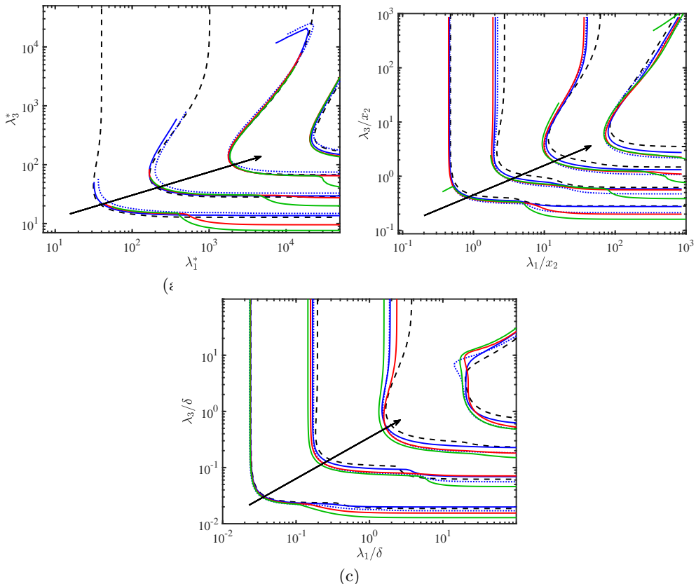
Figure 11: Principal singular value in the relatively subsonic region for (a) c = \bar{u}_{1,\infty}(x_2^* = 10) for the inner layer, (b) c/\bar{u}_{1,\infty} = 0.7 for the logarithmic layer, and (c) c/\bar{u}_{1,\infty} = 0.88 for the outer layer. Contour lines are (a) (10^2, 10^4, 10^6, 10^8)/\sqrt{Re_\tau^* Re_\tau^*} , (b) (10^{-3}, 10^{-1}, 10^1, 10^3) \times x_2^* x_2^* x_2/\delta , and (c) (10^{-7}, 10^{-4}, 10^{-1}, 10^2) \times Re_\tau^* Re_\tau^* . Lines indicate M_\infty = 0 (---), M_\infty = 2 , Re_\tau = 450 (—), M_\infty = 2 , Re_\tau = 900 (.....), M_\infty = 3 (—), and M_\infty = 4 (—). Arrows indicate direction of increasing \sigma_1 .
