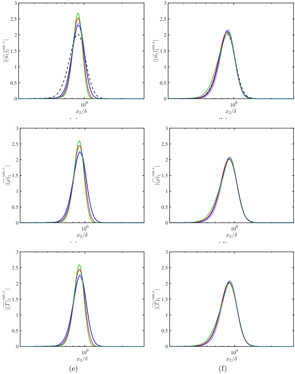
Figure 8: Normalised and scaled response modes in the outer region for streamwise velocity (a) (\widetilde{u}_1)_1^{\text{out},+} and (b) (\widetilde{u}_1)_1^{\text{out},*} , density (c) (\widetilde{\rho})_1^{\text{out},+} and (d) (\widetilde{\rho})_1^{\text{out},*} and temperature (e) (\widetilde{T})_1^{\text{out},+} and (f) (\widetilde{T})_1^{\text{out},*} . Lines indicate M_\infty = 0 (---), M_\infty = 2 , Re_\tau = 450 (—), M_\infty = 2 , Re_\tau = 900 (.....), M_\infty = 3 (—), and M_\infty = 4 (—).
