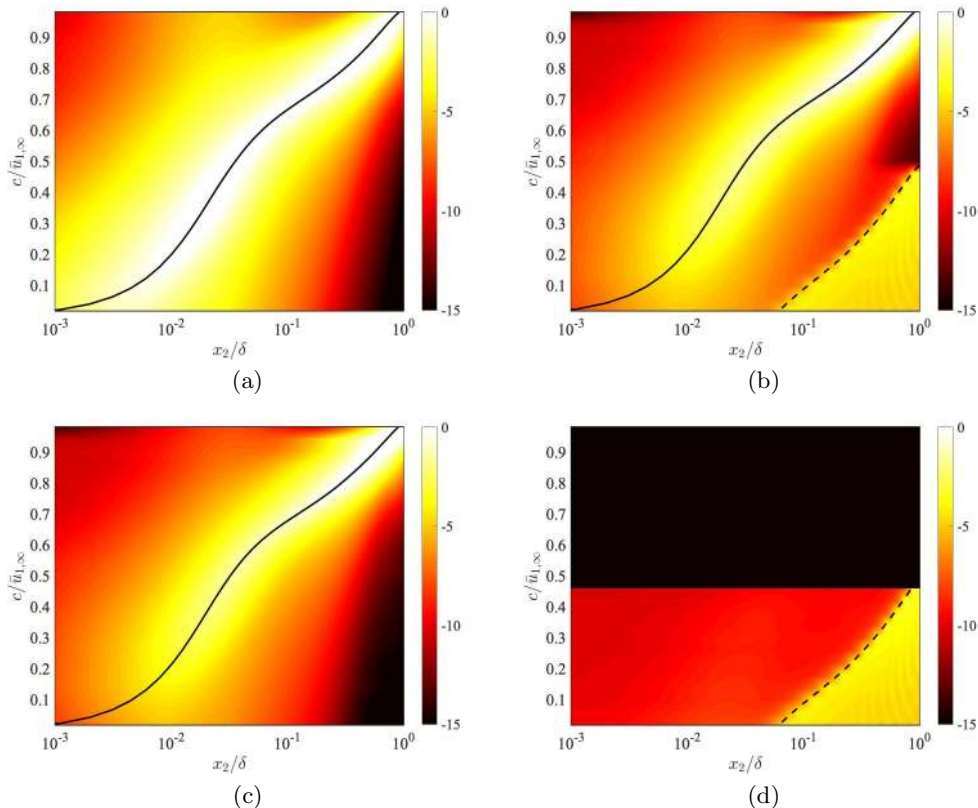
Figure 3: Premultiplied one-dimensional energy density E_{qq} for the (a) incompressible and (b) compressible ( M_\infty = 2 , Re_\tau = 450 ) cases, and the energy density for the compressible case conditionally sampled to (c) \overline{M_\infty} < 1 and (d) \overline{M_\infty} > 1 . The turbulent mean velocity profile, \bar{u}_1 (—) and the relative sonic line \bar{c} (---) are shown for reference. Colours are in logarithmic scale.
