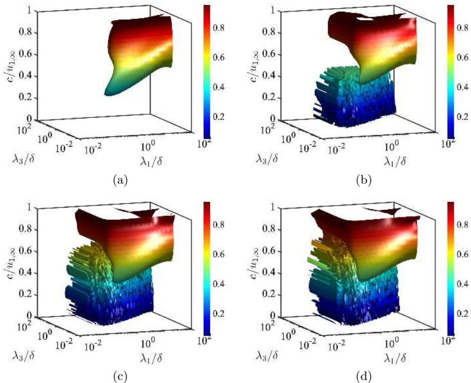
Figure 2: Energy contained in the principal response mode relative to the total response, \sigma_1^2 / (\sum_j \sigma_j^2) , for different streamwise and spanwise wavelengths and wave speeds for the (a) incompressible, (b) M_\infty = 2 , Re_\tau = 450 , (c) M_\infty = 3 and (d) M_\infty = 4 cases. The contour surface is \sigma_1^2 / (\sum_j \sigma_j^2) = 0.75 coloured by wall-normal distance from the wall.
