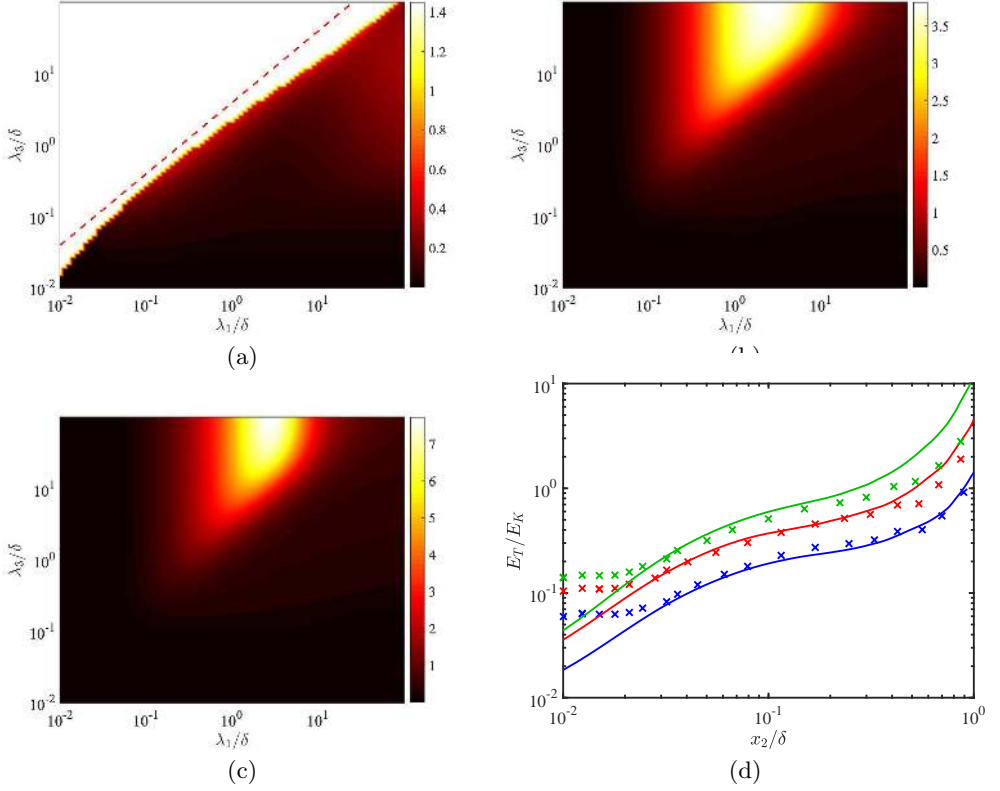
Figure 12: The spectra of the ratio of turbulent thermodynamic and kinetic energy, E_T/E_K computed from the principal resolvent modes at (a) x_2^* = 15 , (b) x_2/\delta = 0.2 and (c) x_2/\delta = 0.5 for the M_\infty = 2 , Re_\tau = 450 case. The relative sonic line \bar{c} (---) is shown for reference. (d) The values of E_T/E_K at the most energetic wave parameters as defined in (4.11) for the principal resolvent modes ( \times ) and DNS (—) for M_\infty = 2 , Re_\tau = 450 (blue), M_\infty = 3 (red), and M_\infty = 4 (green).
