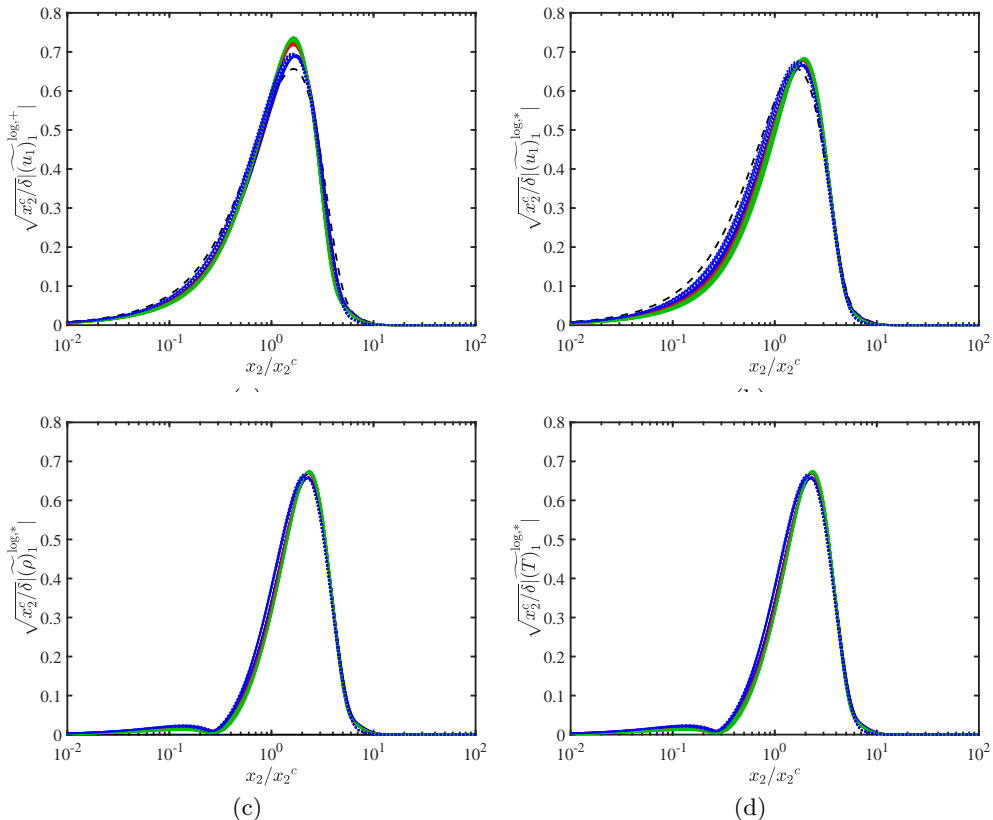
Figure 10: Normalised and scaled response modes in the logarithmic region for streamwise velocity (a) (\widetilde{u}_1)_1^{\text{log},+} and (b) (\widetilde{u}_1)_1^{\text{log},*} , (c) density (\widetilde{\rho})_1^{\text{log},*} and (d) temperature (\widetilde{T})_1^{\text{log},*} scaled by \sqrt{x_2^c} . Lines indicate M_\infty = 0 (---), M_\infty = 2 , Re_\tau = 450 (—), M_\infty = 2 , Re_\tau = 900 (⋯), M_\infty = 3 (—), and M_\infty = 4 (—).
