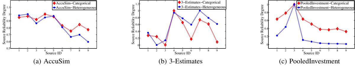
Figure 2: Comparison of Source Reliability Degrees between Methods Applied on Categorical and Heterogeneous Data
