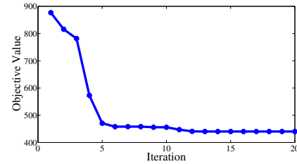
Figure 5: Convergence Rate
