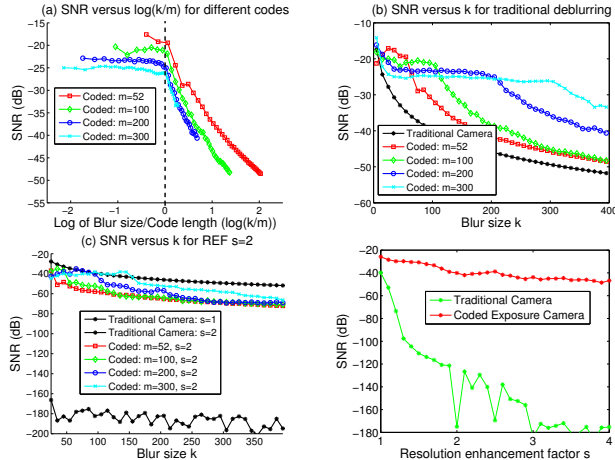
Figure 5. Relationship between code length m , blur size k and REF s . (a) Plots of SNR versus relative blur size k/m for coded exposure camera using codes of different lengths for traditional deblurring ( s = 1 ). Note that for each curve, SNR degrades after k > m . (b) SNR for a coded exposure camera is much better compared to a traditional camera for wide range of code lengths and motion blur sizes. (c) Similar plots as in (b) for combined deblurring and resolution enhancement ( s = 2 ), showing that it is impractical using a traditional camera. (d) SNR versus s for a fixed blur size k ( = 100 ) pixels and object size n ( = 25 ) pixels. As s increases, reconstruction noise also increases.
