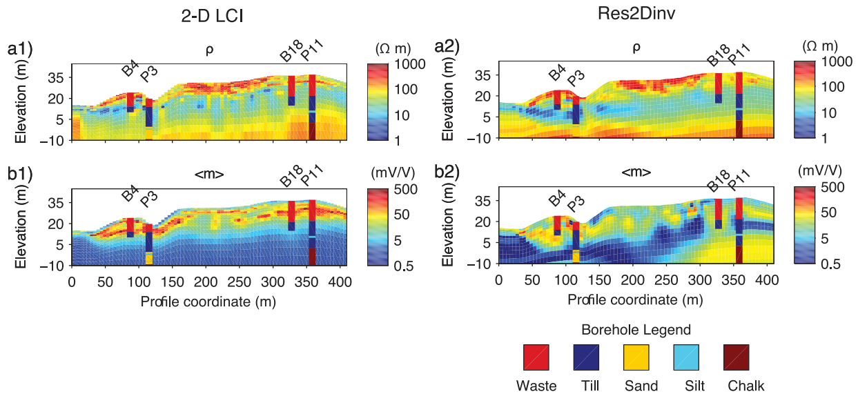
Figure 7. Comparison of 2-D LCI and Res2Dinv inversions, in terms of resistivity and integral chargeability sections. The 2-D LCI integral chargeability section has been derived from the Cole–Cole parameters shown in Fig. 5.
