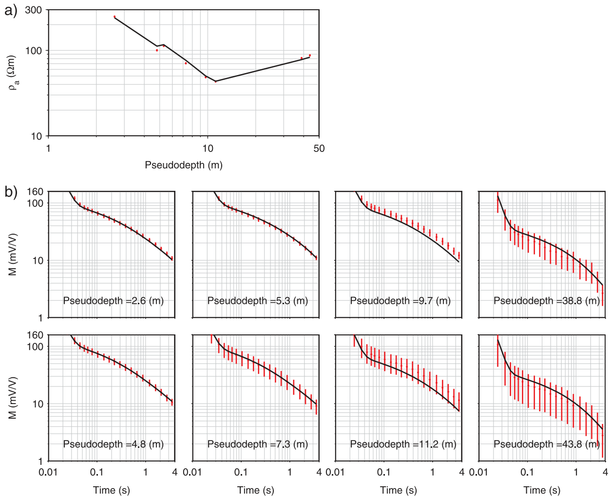
Figure 6. Data fit of Fig. 5 inversion for the quadrupoles of the acquisition sequence with lateral focus between 245 and 250 m along the profile. (a) Apparent resistivity data fit; b) chargeability data fit. Red lines: data with error bars. Black lines: data fit.
