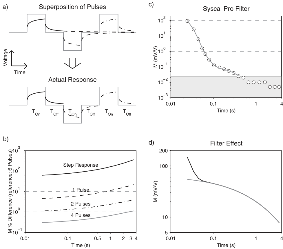
Figure 1. (a) Construction of the pulse response by superimposing two-step responses; (b) IP percentage difference between decays with different number of stacks (a decay stacked six times is used as a reference) for the homogeneous half-space described by the Cole–Cole parameters ( m_0 = w 100 \text{ mV V}^{-1} , \tau = 2 \text{ s} , c = 0.5 ). Solid black line, step response; dashed line, 1 pulse; dotted-dashed line, 2 pulses; grey solid line, 4 pulses. The on- and off-times used for the waveform are: T_{on} = T_{off} = 4 \text{ s} . Note that the per cent axis is logarithmic. (c) IRIS Syscal Pro filter effect (circles) measured in the time domain on a non-chargeable resistor. The grey line represents the modelling of the filter, for which the measurements in the grey rectangle have not been taken into account (because the limit of the digitization of the data has been reached). (d) Example of forward response with the filter implementation (black line) and without the filter implementation (grey line).
