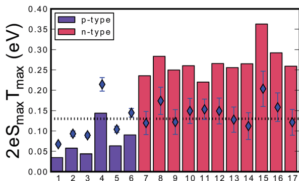
Fig. 6 Estimation of the band gap for different n-type (red bars) and p-type (purple bars) half-Heusler compounds using the Goldsmid–Sharp formula ( E_g = 2eS_{max}T_{max} ) in units of eV versus the numerated HH compounds. The dotted line indicates the optical measured band gap of 0.13 eV for pure ZrNiSn from DRIFTS. The diamonds represent the estimated true band gap value that yields the experimental S_{max} and T_{max} when using the full relation derived by Goldsmid and Sharp for an electron-to-hole weighted mobility ratio of A = 5 : (1) Sc_{0.03}Zr_{0.97}NiSn , (2) Sc_{0.04}Zr_{0.96}NiSn , (3) Sc_{0.05}Zr_{0.95}NiSn , (4) Sc_{0.1}Zr_{0.9}NiSn , (5) ZrCo_{0.08}Ni_{0.92}Sn , 22 (6) ZrCo_{0.12}Ni_{0.88}Sn , 22 (7) Zr_{0.75}Hf_{0.25}NiSn , 42 (8) Zr_{0.5}Hf_{0.5}NiSn , 42 (9) Zr_{0.25}Hf_{0.75}NiSn , 42 (10) HfNiSn , 42 (11) Ti_{0.95}Hf_{0.05}NiSn , 43 (12) Ti_{0.95}Hf_{0.05}NiSn_{0.995}Sb_{0.005} , 43 (13) Ti_{0.95}Hf_{0.05}NiSn_{0.99}Sb_{0.01} , 43 (14) Ti_{0.95}Hf_{0.05}NiSn_{0.98}Sb_{0.02} , 43 (15) Hf_{0.75}Zr_{0.25}NiSn_{0.99}Sb_{0.01} , 44 (16) Hf_{0.5}Ti_{0.25}Zr_{0.25}NiSn_{0.99}Sb_{0.01} , 44 and (17) Hf_{0.25}Ti_{0.5}Zr_{0.25}NiSn_{0.99}Sb_{0.01} . 44
