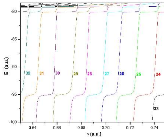
Figure 2. Enlarged view of the Stabilization diagram for ^1S^e states of exotic pKK ion below N = 2 ionization threshold of pK
