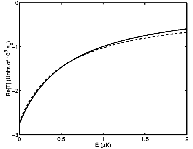
FIG. 4. Comparison of the real part of the T matrix for coupled square-well scattering (solid line) with a potential range R = 1a_0 , to Feshbach scattering (dashed line), for a detuning that yields a scattering length of about -2750a_0 . A similar, good agreement is found for all detunings.
