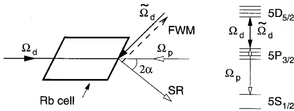
Figure 2. Experimental set-up to study four-wave-mixing process on the interface between glass and rubidium vapour.
