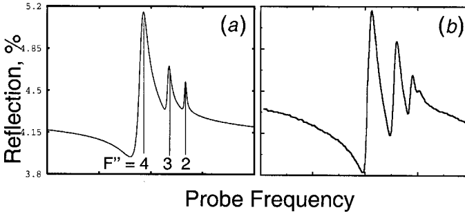
Figure 4. Calculated (a) and experimental (b) selective reflection spectrum when the probe frequency is swept in the area red shifted ( \sim 800 MHz) from the D 2 line of ^{87}\text{Rb} ( F = 2 \rightarrow F' ). The drive frequency is fixed and tuned to the 5P_{3/2} , F' = 3 \rightarrow 5D_{5/2} transition of ^{87}\text{Rb} . Observed resonances correspond to the fine structure of the 5D_{5/2} state. Incident angle is equal to \alpha = 0.1 rad.
