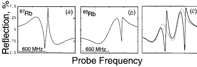
Figure 3. Calculated (a, b) and experimental (c) selective reflection spectrum when the probe frequency is swept around D 2 line of ^{85}\text{Rb} ( F = 3 \rightarrow F' ) and ^{87}\text{Rb} ( F = 2 \rightarrow F' ). The drive frequency is fixed and tuned to the 5P_{3/2} , F' = 3 \rightarrow 5D_{5/2} , F'' = 4 transition of ^{87}\text{Rb} . Dotted experimental curve (c) shows the reflection spectrum without the driving field. Incident angle is equal to \alpha = 0.1 rad.
