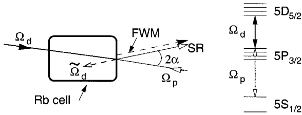
Figure 1. Experimental set-up and scheme of atomic levels.
