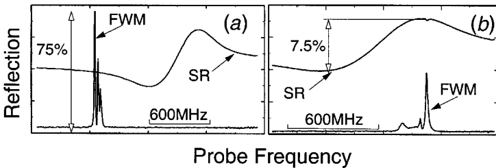
Figure 5. Selective reflection and four-wave-mixing spectra for the configuration shown in figure 2. (a) The drive field is red shifted ( \sim 950 MHz) and (b) the drive field is blue shifted ( \sim 300 MHz) from the 5P_{3/2} , F' = 3 \rightarrow 5D_{5/2} transition of ^{87}\text{Rb} . Forward \Omega_d and backward \tilde{\Omega}_d drive fields have the same intensity and polarization. Incident angle is set to Brewster's angle. Vertical scales for both pictures are the same.
