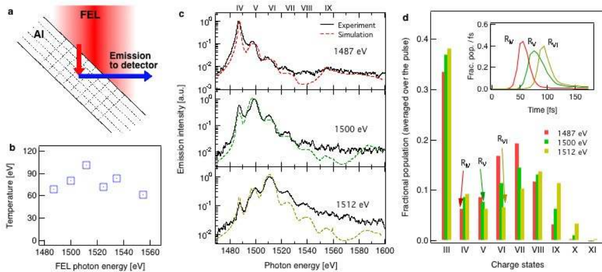
FIG. 2. (a) Geometrical consideration for SCFLY simulations. Each cell (100 nm \times 100 nm \times 100 nm) in the sample receives the X-ray flux based on the intensity profile of focal spot and transmission by preceding layers. Emission from each cell is reabsorbed by other cells in the line of sight to the detector. (b) Calculated electron temperatures at the end of X-ray pulse. (c) Calculated emission spectra (color dashed) at the first three resonances are compared with experiment (black solid). (d) Average CSD over the duration of X-ray pulse. (Inset) Temporal evolution of R_{IV} , R_V and R_{VI} , which are resonant states with 1487 eV, 1500 eV and 1512 eV photon energies, respectively.
