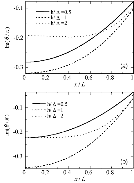
FIG. 4. Spatial dependence of \text{Im } \theta for majority spin for R_d/R'_b=0.1 , E_{Th}/\Delta=1 and various h/\Delta with (a) R_d/R_b=5 and (b) R_d/R_b=10 . The DF/N interface and the DF/S interface are located at x=0 and x=L respectively.
