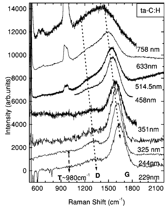
FIG. 2. MW Raman spectra of a ta-C:H sample with \sim 70\% sp^3 and \sim 30\% H. The G and D peaks' dispersions are indicated. The T peak at \sim 980\text{ cm}^{-1} is also shown. Note that it does not disperse excitation energy, but just rapidly falls in intensity with decreasing excitation energy, as expected for an sp^3 VDOS. For the lower excitation energies the contributions from the Si first- and second-order modes are also seen (Ref. 67).
