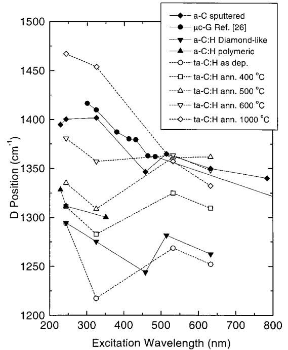
FIG. 15. Dispersion of D peak vs excitation wavelength for a series of representative samples. The series of ta-C:H, as deposited and annealed at various temperatures, is marked by dotted lines. Data on microcrystalline graphite from Pocsik et al. (Ref. 26) are added for completeness. Note that there is no D peak for ta-C at any wavelength.
