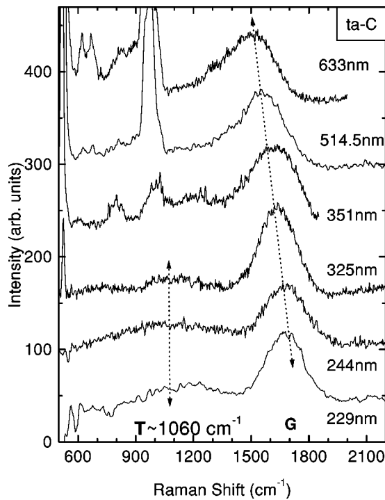
FIG. 1. MW Raman spectra of a ta-C sample with \sim 88\% sp^3 . The G peak dispersion is indicated. The T peak at \sim 1060\text{ cm}^{-1} is also shown; note that it does not disperse excitation energy, but just rapidly falls in intensity with decreasing excitation energy, as expected for an sp^3 VDOS. Note also the double structure which is evident at 325 nm excitation, with a lower frequency peak at \sim 600\text{ cm}^{-1} (see text). For the lower excitation energies the contributions from the Si first- and second-order modes are also seen (Ref. 67).
