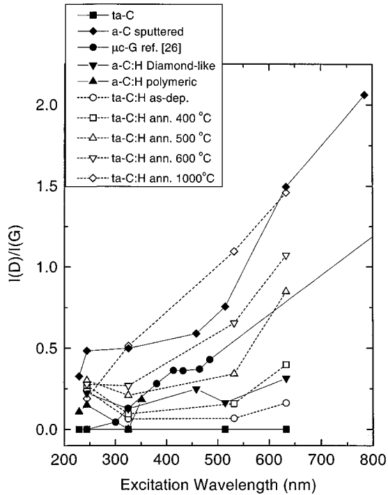
FIG. 14. Dispersion of I(D)/I(G) vs excitation wavelength for a series of representative samples. The series of ta-C:H, as deposited and annealed at various temperatures is marked by dotted lines. Data on microcrystalline graphite from Pocsik et al. (Ref. 26) are added for completeness.
