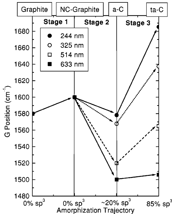
FIG. 11. Amorphization trajectory, showing the schematic variation of G position for four typical wavelengths.
