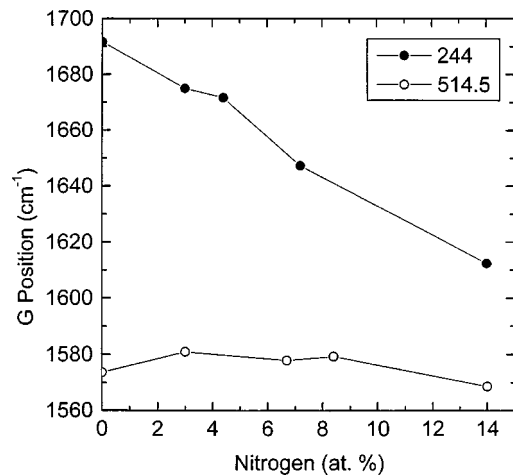
FIG. 13. G peak position (measured at 244 and 514.5 nm) vs nitrogen content (at. %) for ta-C:N samples deposited with a S -bend FCVA (Ref. 42). The nitrogen content was estimated from XPS (Ref. 42). Note that to an almost zero change of the G peak position at 514.5 nm, corresponds an almost linear decrease with N at 244 nm. This is a clear example of inversion (see text). MW Raman spectroscopy of N containing samples will be discussed in detail elsewhere.
