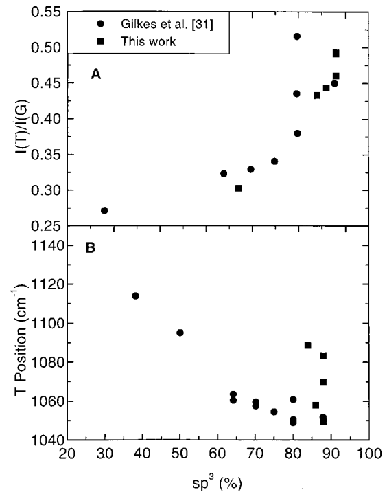
FIG. 19. (a) I(T)/I(G) vs sp^3 fraction for nonhydrogenated carbon films. (b) T peak position vs sp^3 fraction for nonhydrogenated carbon films. The parameters were derived with a BWF+Lorentzian fit, thus allowing the T peak to upshift, as for Gilkes et al. (Ref. 31). A higher T peak position for a given sp^3 content means higher clustering of the sp^2 phase (see text).
