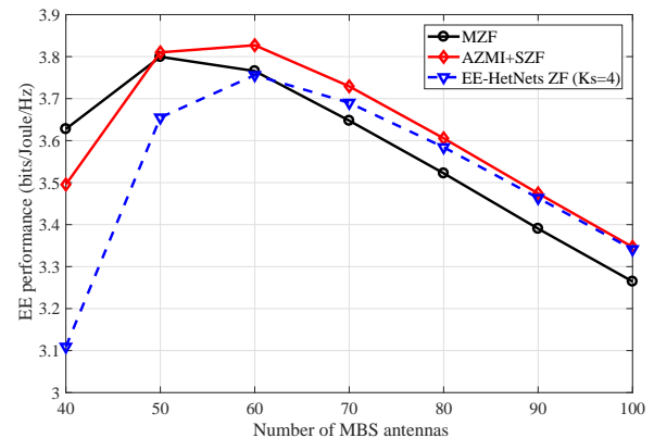
Figure 2. The EE performance versus the number of MBS antennas in a scenario of massive MIMO HetNets. Circle cell structure with radius 1000 m is setup with a centrally located MBS equipped with large-scale antennas, 6 SBSs equipped with 4 antennas and > 30 single-antenna users randomly distributed. Other simulation parameters are as follows: carrier frequency = 2 GHz, Bandwidth = 10 MHz, MBS and SBSs transmission power = 46 dBm and 30 dBm, path-loss model of MBS and SBS 128.1 + 37.6 \log_{10} R dB and 140.7 + 36.7 \log_{10} R dB ( R in km), noise power density -174 dBm/Hz. The throughput threshold per user is 4 Mbps.
