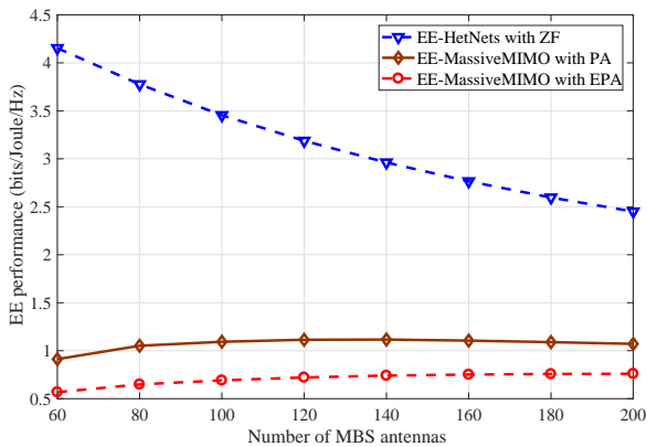
Figure 3. The EE performance versus the total number of antennas in a HetNet scenario. Energy efficiency zero-forcing for HetNets and massive MIMO beamforming are employed. The throughput threshold per user is 4 Mbps.
