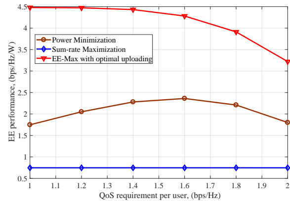
Figure 1. The average EE performance versus per-user QoS threshold. Circle cell structure with radius 250 m is setup with a MBS equipped with 10 antennas at centrally coverage network, 4 SBSs equipped with 2 antennas and 14 single-antenna users randomly distributed. Other simulation parameters are as follows: carrier frequency = 2 GHz, Bandwidth = 10 MHz, transmit power of MBS and SBSs = 43 dBm and 30 dBm, path-loss of MBS and SBS 128.1 + 37.6 \log_{10} R dB and 140.7 + 36.7 \log_{10} R dB ( R in km), noise power density -174 dBm/Hz.
