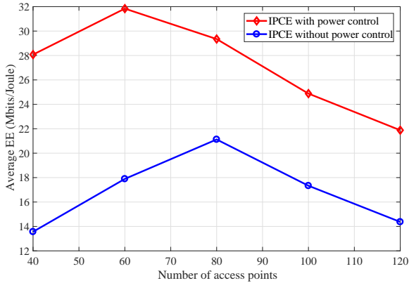
Figure 4. The average EE performance versus the number of access points. A wrapped around cell structure with 1 \times 1 \text{ km}^2 is setup with 16 single-antenna users randomly distributed. The coefficient models of large-scale fading is as COST Hata model. The carrier frequency f_c = 1.9 \text{ GHz} , bandwidth B = 20 \text{ MHz} , \tau = 200 , maximum transmit power of each AP and user are 200 and 100 mW. The noise power at the receivers is N_0 = 290 \times \kappa \times B \times NF , where \kappa and NF are Boltzmann constants and noise figure at 9 dB.
