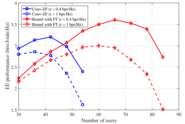
Figure 5. EE performance of a three-cell network versus the number of users per cell. Hexagonal cell structure with radius 1 km is setup with a centrally located BS equipped with 8 \times 8 uniform planar array of antennas. Standard exponential correlation model is assumed to implement antenna spatial correlation with correlation factor of 0.9. Other simulation parameters are as follows: carrier frequency = 2 GHz, Bandwidth = 10 MHz, BS transmission power = 46 dBm, path-loss model 128.1 + 37.6 \log_{10} R \text{ dB} ( R in km), noise power density -174 \text{ dBm/Hz} .
