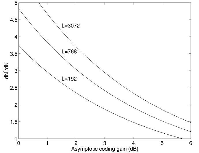
Fig. 6. dN^*/dK versus asymptotic coding gain ( 10 \log \beta ).
