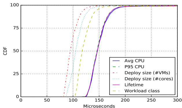
Figure 10: Latency of model execution for our metrics.
