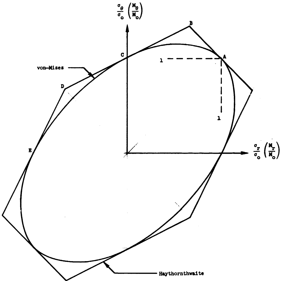
Figure 3. - Yield surfaces for von-Mises and Haythornthwaite yield conditions for plane stress problems.
