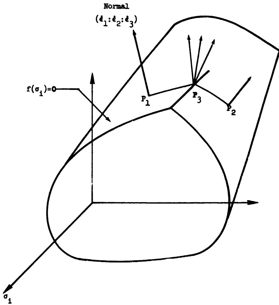
Figure 1. - Generalized yield conditions and flow rules.
