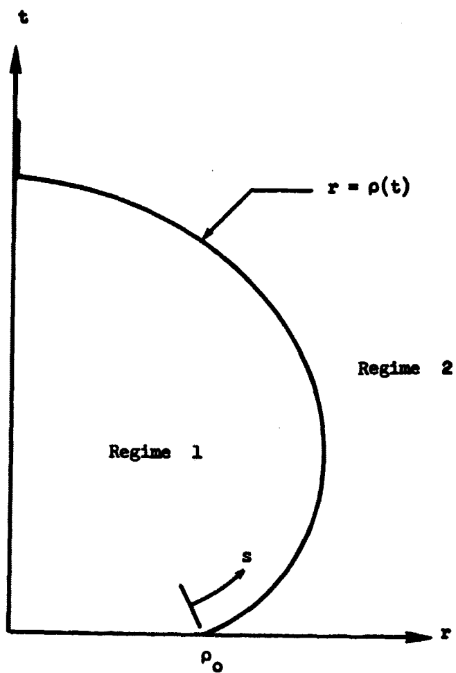
Figure 5. - General motion of a circle of discontinuity.
