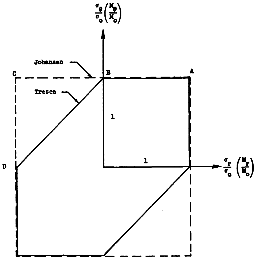
Figure 4. - Yield surfaces for Tresca and Johansen yield conditions for plane stress problems.
