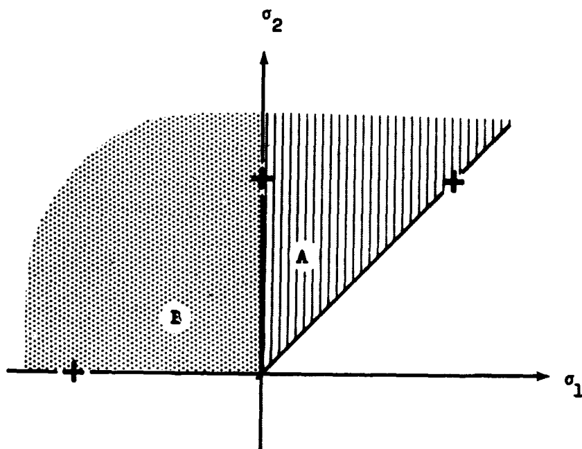
Figure 2. - Yield regions determined by boundary conditions in plane stress problems for circular plates.
