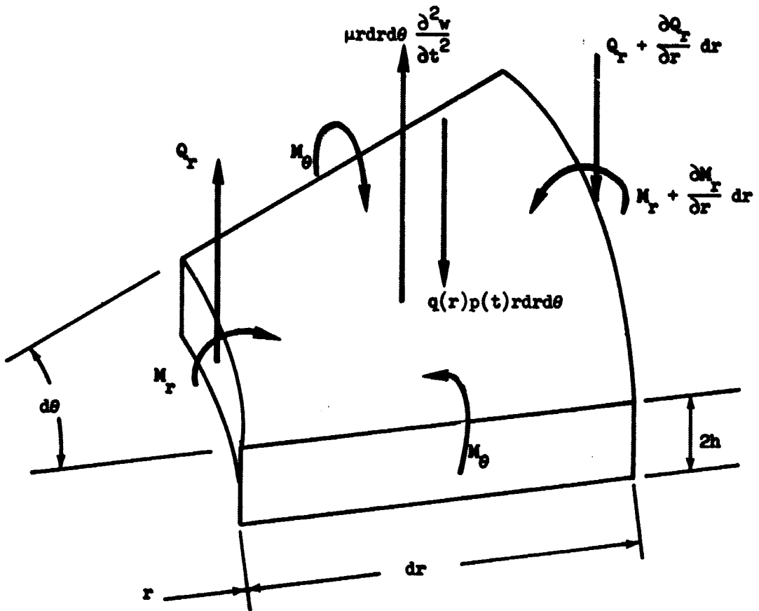
Figure 6. - Applied forces and moments on plate element.
