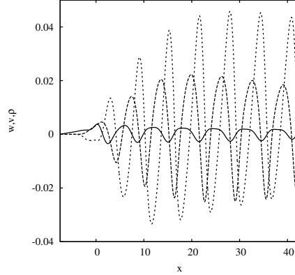
FIGURE 4. Streamwise profile of the normal velocity w (solid line), transverse velocity v (dashed line) and density \rho (dotted line) at z_c = 0.75 . Re = 593 , F = 1.046 , k = 1.041 , \alpha = \pi/4 and h = 0.06
