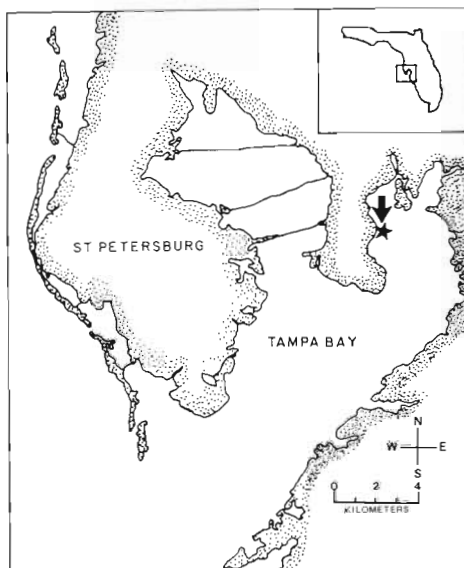
Fig. 1. Location of study area in Hillsborough Bay, Tampa, Florida, USA. Arrow denotes sample site
