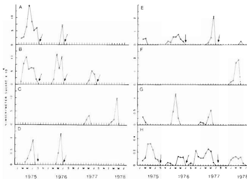
Fig. 4. Response of dominant species in Hillsborough Bay during study period. A: Mysella planulata ; B: Ampelisca abdita ; C: Streblospio benedicti ; D: Grandidierella bonnieroides ; E: Mulinia lateralis ; F: Mediomastus californiensis ; G: Cyclaspis sp.; H: Nereis succinea
