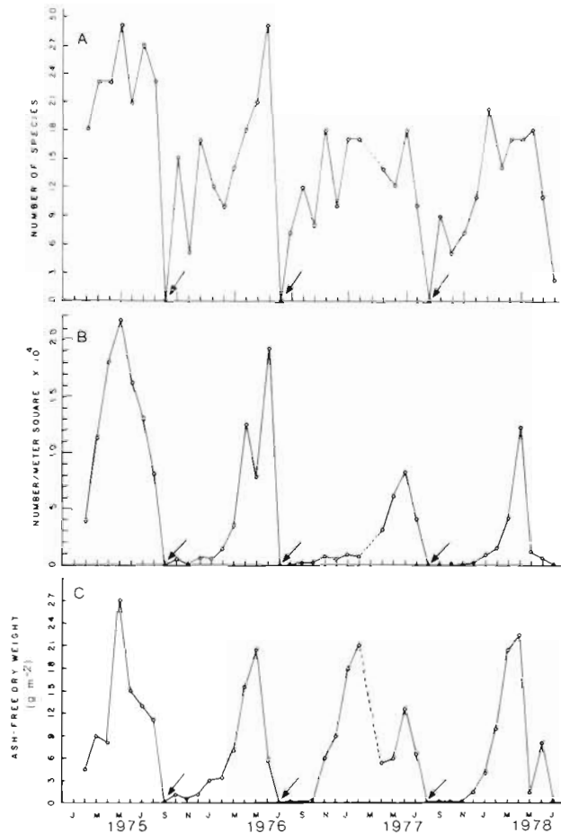
Fig. 3. Total faunal response in Hillsborough Bay during study period. A: Number of species, B: total density (# m -2 ); C: total biomass (g dry wt. m -2 ). Arrows indicate periods of defaunations; broken lines indicate interpolated data
