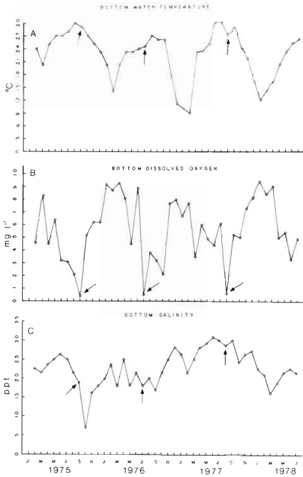
Fig. 2. Environmental parameter measurements in Hillsborough Bay during study period. Arrows indicate periods of defaunations
