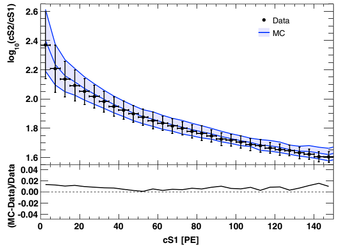
FIG. 7 (color online). Two-dimensional distributions of the means of the single-scatter elastic nuclear recoil population from ^{241}\text{AmBe} calibration data (black) and MC simulation (blue), where \log(\text{cS2}/\text{cS1}) is the discrimination parameter and the energy scale is defined by the primary scintillation channel (top). The error bars (black) and filled area (blue) represent the \pm 1\sigma bands for the data and MC simulation respectively. The bottom panel shows the residual differences between the data and MC simulation which are all within 2%.
