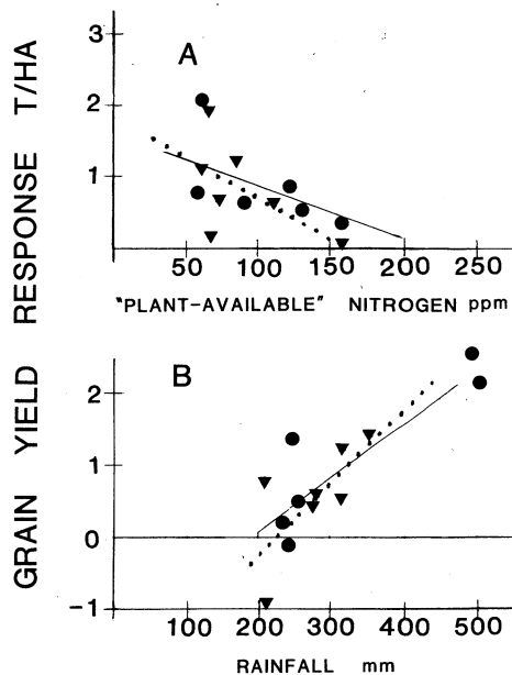
Figure 3: A. Relationship between grain yield response to nitrogen fertiliser adjusted to a mean spring-summer rainfall of 305 mm, and soil concentrations of 'plant-available' nitrogen for shallow soils (●) ..... and deep soils (▼) ———. B. Relationship between grain yield response to nitrogen fertiliser adjusted to a mean soil concentration of 'plant-available' nitrogen of 95 ppm, and spring-summer rainfall for shallow soils (●) ..... and deep soils (▼) ———.
