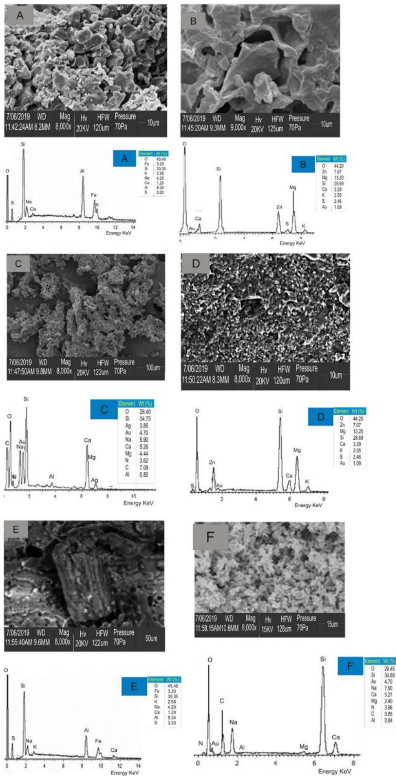
Fig. 2 SEM and EDX images of raw and amended soil samples. Group A water (control), group B: 100 mg \text{Ca}(\text{NO}_3)_2/\text{kg} soil, group C: 100 mg \text{CaNPs}/\text{kg} soil, group D: 75 mg \text{CaNPs}/\text{kg} soil, group E: 50 mg \text{CaNPs}/\text{kg} soil, F- pre-planting (raw) soil
