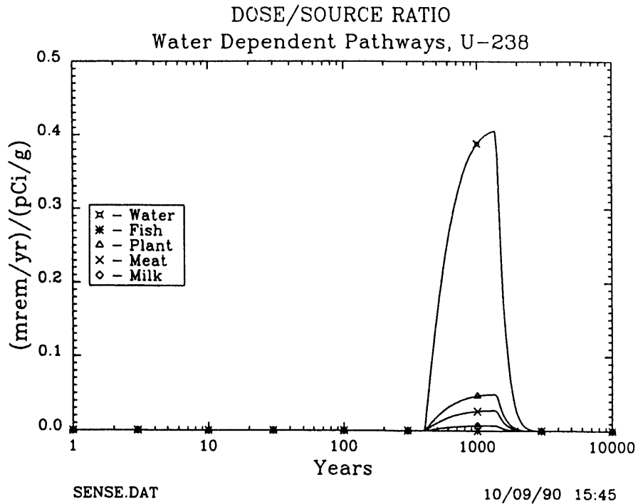
FIGURE 4 Dose/Source Ratio of Water-Dependent Pathways of Uranium-238
