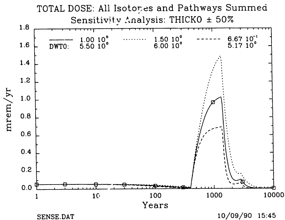
FIGURE 7 Total Dose of All Isotopes Summed over All Pathways with Sensitivity Analysis of THICK0
