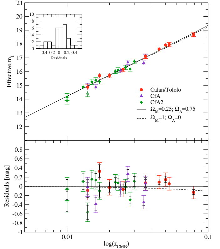
Fig. 7. Effective I -band maximum vs. redshift for the nearby supernovae of the Calan/Tololo, CFA and CFA2 sample. The data have been corrected for the stretch-luminosity relation and for Milky Way and host galaxy extinction. The rms along the concordance model line is \sigma = 0.17 \pm 0.04 \text{ mag} . Subtracting the contribution of the average uncertainty, results in 0.13 \text{ mag} estimated intrinsic dispersion (see text for details). SN 1998es and SN 1999dq were excluded from the fit (see text) and are plotted with open diamonds. The inset plots the histogram of the residuals.
