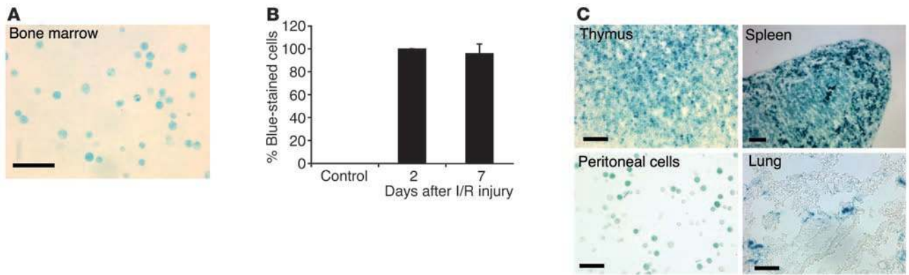
Figure 6 Confirmation of chimerism in mice transplanted with \beta -gal-expressing bone marrow. (A) Fixed bone marrow cells stained blue with X-gal. (B) Percentage of bone marrow cells that stained blue with X-gal in control C57BL/6J mice and chimeric mice ( n = 5 per time point) subjected to I/R followed by 2 days and 7 days of recovery. (C) Peritoneal cells as well as cells of thymus, spleen, and lung from chimeric mice all stained positively with X-gal. Scale bars: 50 \mu m.
