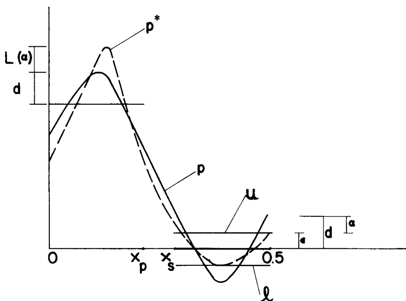
FIGURE 1. Constrained approximation p^* is shown with unconstrained approximation p . \alpha is the gain and L(\alpha) the loss due to the restraining lines in the stopband
