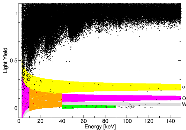
Fig. 9 The data of detector module Ch51, shown in the light yield vs. recoil energy plane. Again, the shaded areas indicate the bands, where alpha ( yellow ), oxygen ( violet ), and tungsten ( gray ) recoil events are expected. Additionally highlighted are the acceptance region ( orange ), the region where lead recoils with energies between 40 and 90 keV are expected ( green ), and the events observed in these regions. The highlighted lead recoil region ( green ) serves as a reference region for estimating the ^{206}\text{Pb} recoil background (Color figure online)
