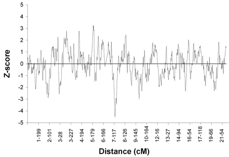
Figure 1. Genomewide admixture mapping results in 482 men with prostate cancer, adjusted for age
