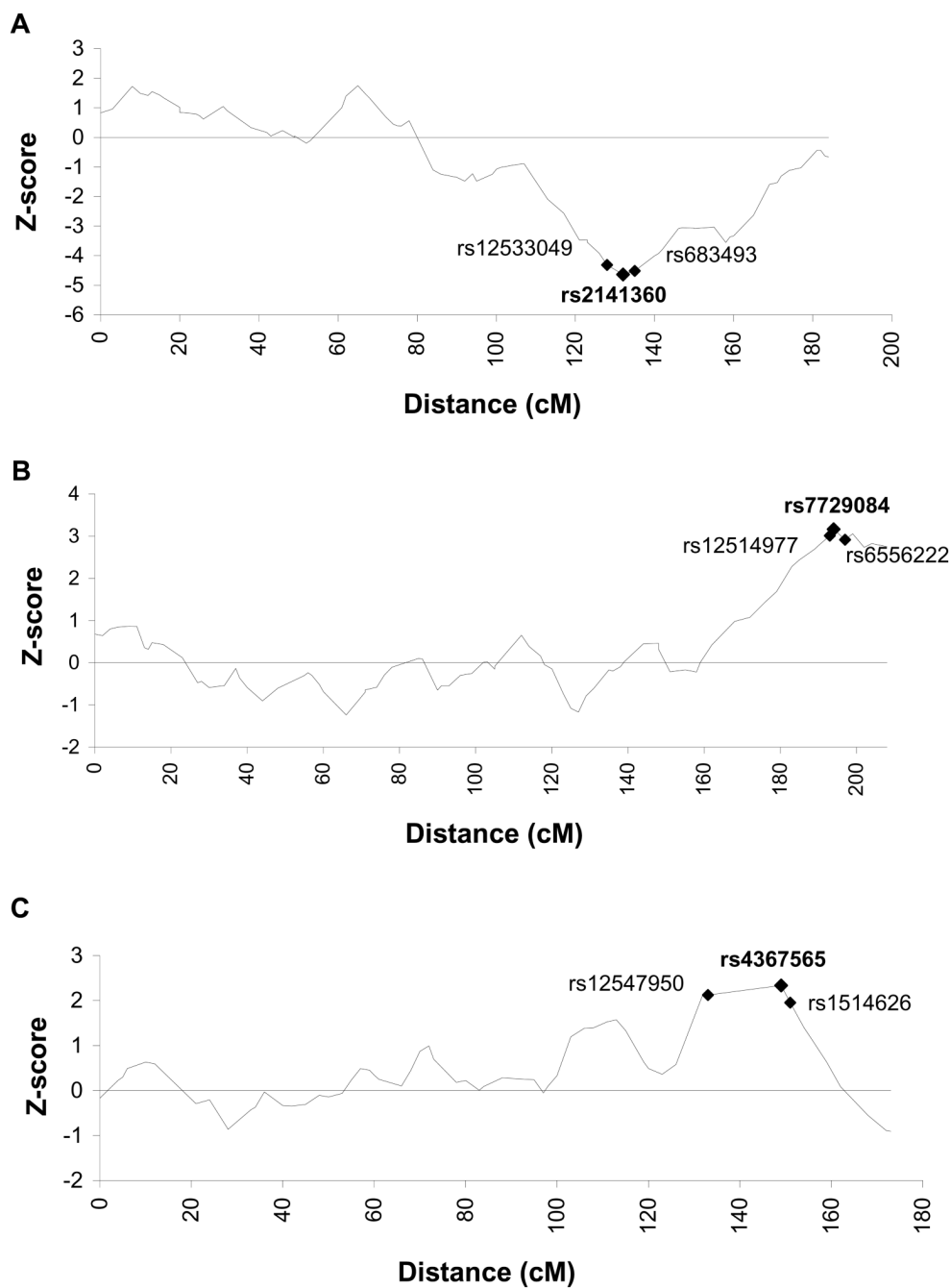
Figure 2. Admixture mapping results from select chromosomes in 482 African American men with prostate cancer, adjusted for age. (A) Chromosome 7 (B) Chromosome 5 (C) Chromosome 8
