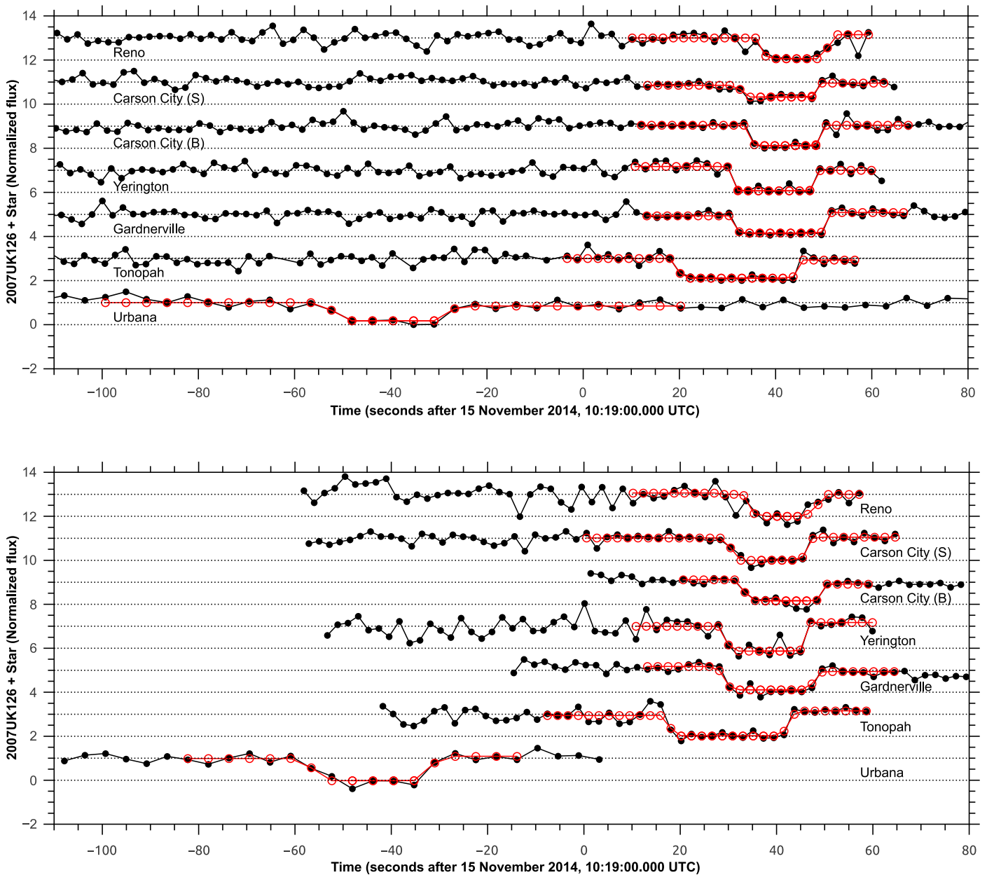
Figure 2. Top panel: the seven occultation light curves, obtained from the GBR extraction (see text), normalized to the unocculted star plus 2007 UK 126 flux and vertically shifted by integer values for better viewing. The red lines and circles are the square-well model convoluted by the Fresnel diffraction, the star apparent angular diameter, and the finite exposure time. The mid-times of the occultations do not coincide due to the propagation delays of the shadow due to the distinct longitudes of the sites (Figure 1). Bottom panel: same from the MWB extraction. Note that no secondary occultation is observed, as could be caused by a satellite.
