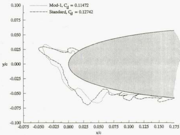
Figure 12.—Comparison of ice shape obtained from standard and Mod-1 nozzles for \alpha = 4^\circ , V_\infty = 230 mph, T_t = 22^\circ\text{F} , LWC = 1.0 g/m 3 , MVD = 30 \mu\text{m} , t = 6 min.
