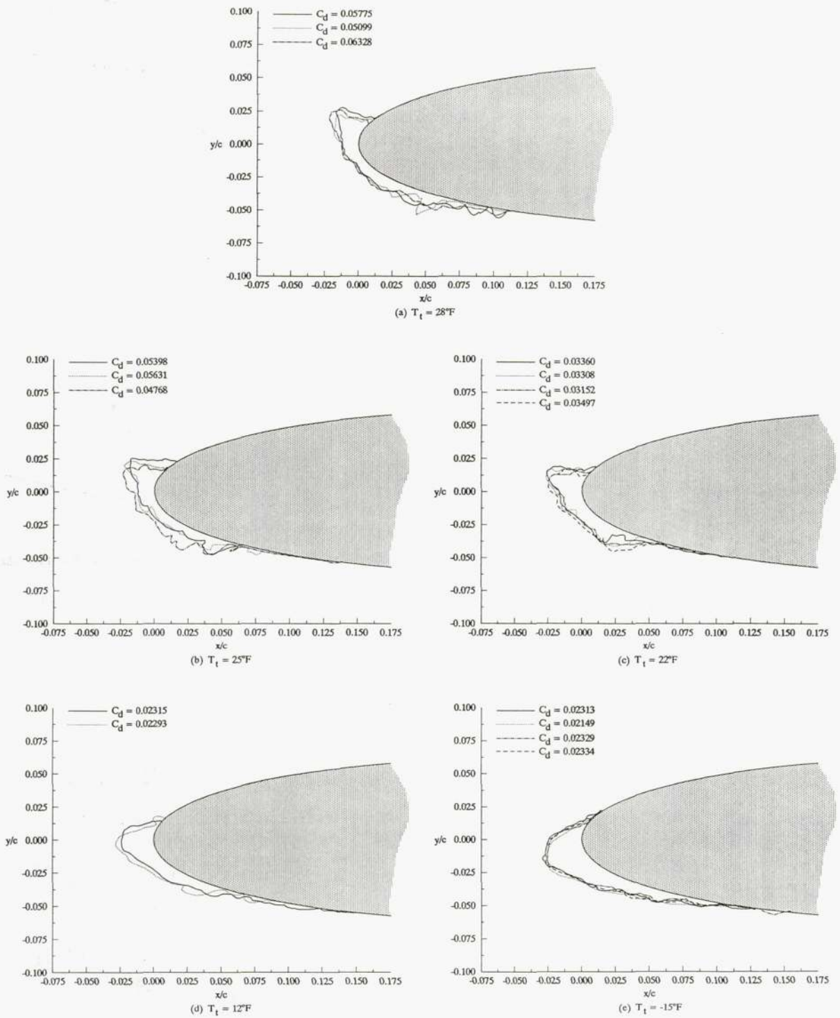
Figure 6.—Repeatability of ice shape and drag coefficient with total air temperature for \alpha = 4^\circ , V_\infty = 150 mph, LWC = 1.0 g/m 3 , MVD = 20 \mu\text{m} , t = 6 min.
