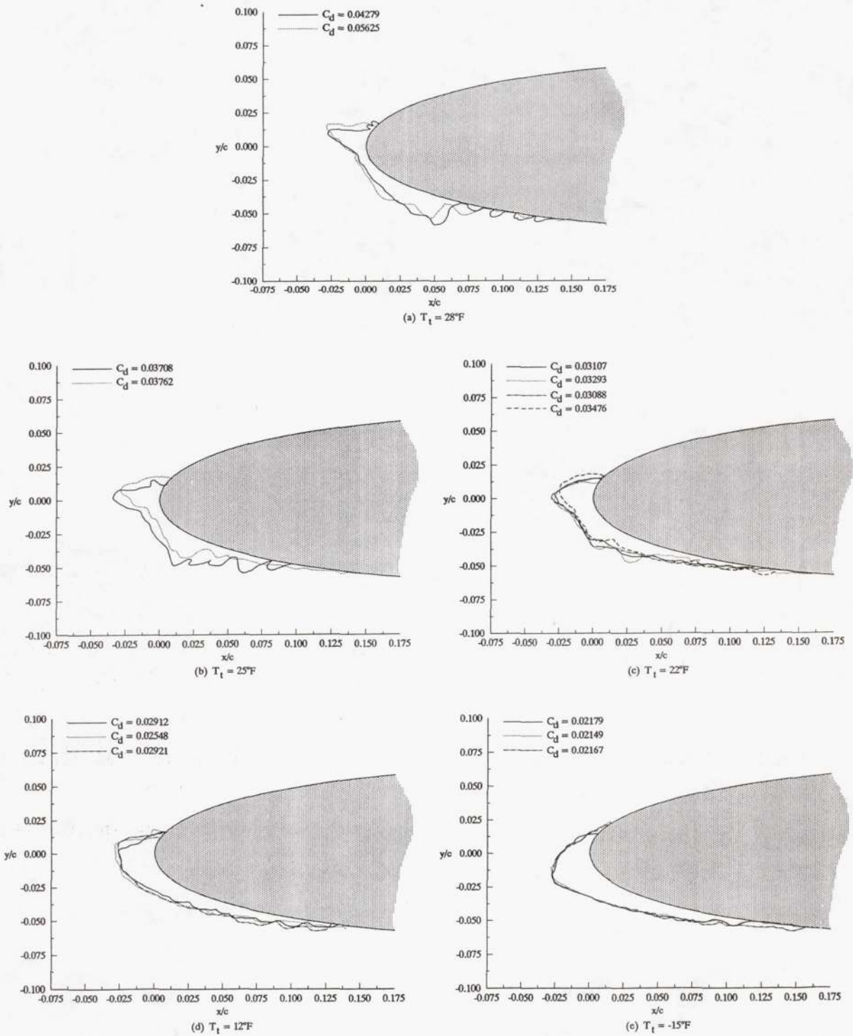
Figure 7.—Repeatability of ice shape and drag coefficient with total air temperature for \alpha = 4^\circ , V_\infty = 230 mph, LWC = 0.55 g/m 3 , MVD = 20 \mu m, t = 7 min.
