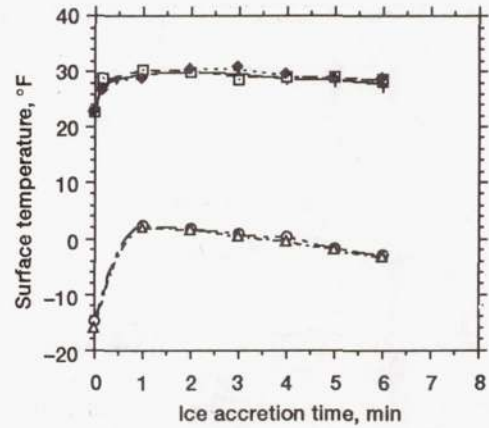
Figure 19.—Repeatability of model surface temperature of the leading edge at mid-span for total air temperatures of 22 and -15^\circ\text{F} ( \alpha = 4^\circ , V_\infty = 150 mph, LWC = 1.0 \text{ g/m}^3 , MVD = 20 \mu\text{m} ).
