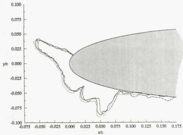
Figure 10.—Comparison of ice shape taken by three data takers ( \alpha = 4^\circ , V_\infty = 230 mph, T_t = 22^\circ\text{F} , LWC = 1.3 g/m 3 , MVD = 30 \mu\text{m} , t = 6 min).
