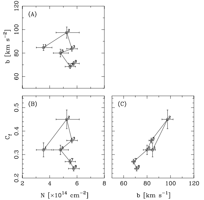
FIG. 6.—Relationship between (a) column density and Doppler parameter, (b) column density and coverage fraction, and (c) Doppler parameter and coverage fraction, with 1\sigma error bars for the narrow component of the C IV mini-BAL in system A. Each point is labeled with the epoch number.
