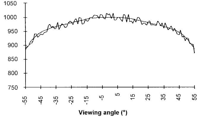
Fig. 10. Typical response on a radial section of the CCD ( p^k \cdot gm f_{lp}^k \cdot gh f_{lp}^k ). The smooth line represents the low-frequency variation of multiangular calibration p^k .
