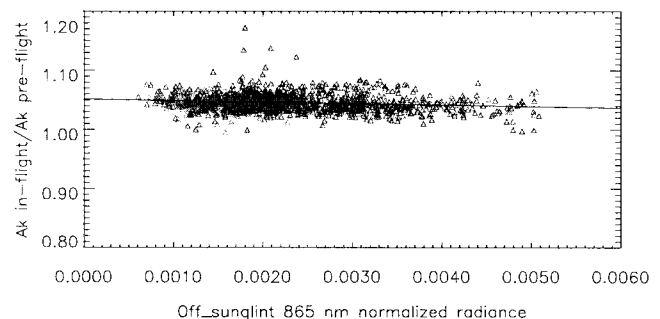
Fig. 8. Absolute calibration elementary results for sunglint interband method as a function of the Rayleigh corrected 865-nm radiance in an off-sunglint direction (for all the calibration points selected during the first week of November 1996). Correlation with the aerosol content is very small: this validates the aerosol effect correction. The Sunglint method is 865 nm.
