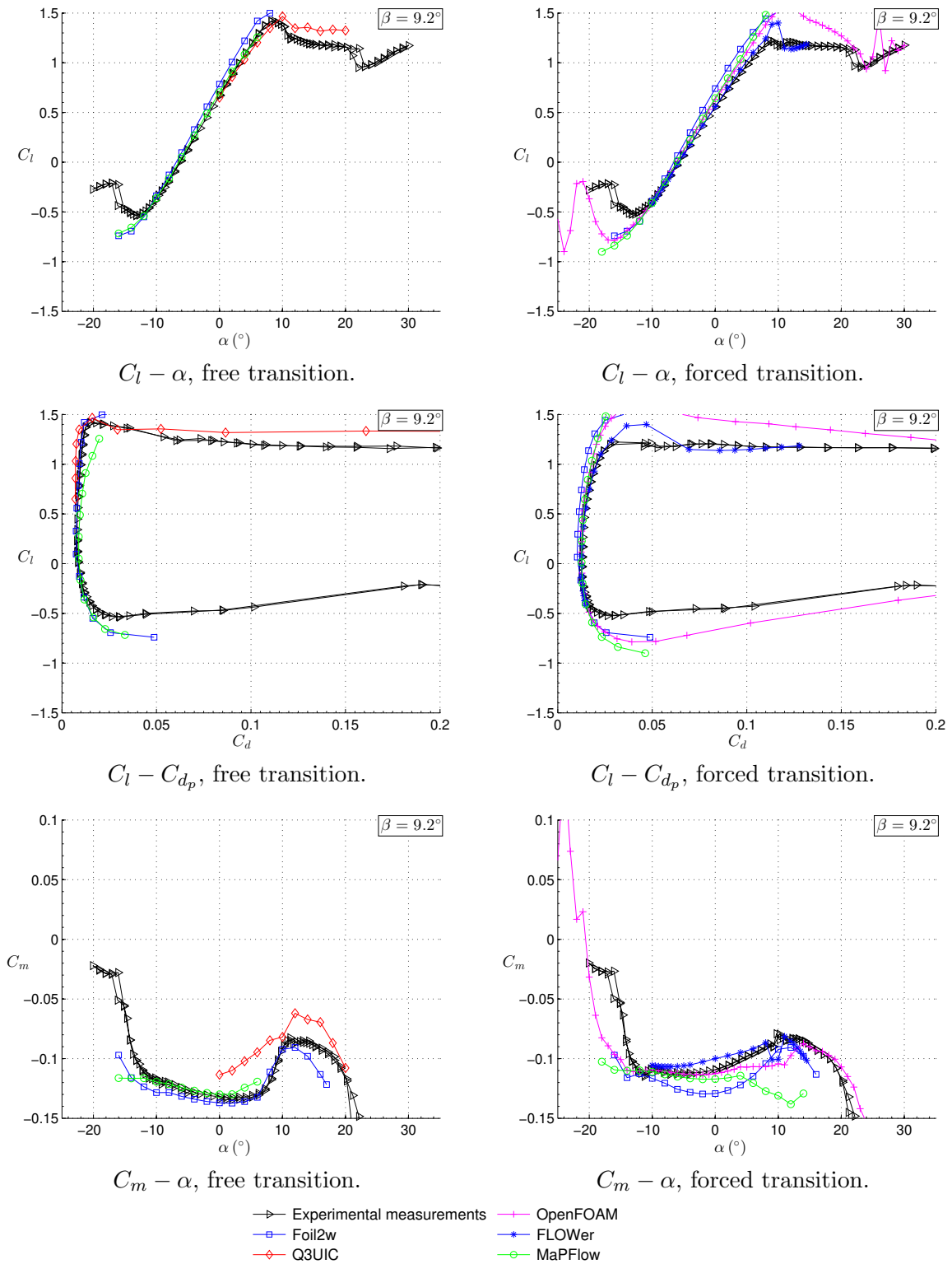
Figure 2. Validation of the numerical simulations with the steady experimental polars of the DU95W180 airfoil for varying angle of attack and fixed flap angle ( C_l - \alpha , C_l - C_{d_p} , C_m - \alpha ) at Re \approx 1.0 \times 10^6 , with free and forced transition, for \beta = 9.2^\circ and -20^\circ < \alpha < 30^\circ (cases STDY5 and STDY10).
