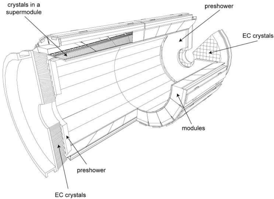
Figure 1: Layout of the CMS electromagnetic calorimeter showing the arrangement of crystal modules, supermodules and end-caps.
