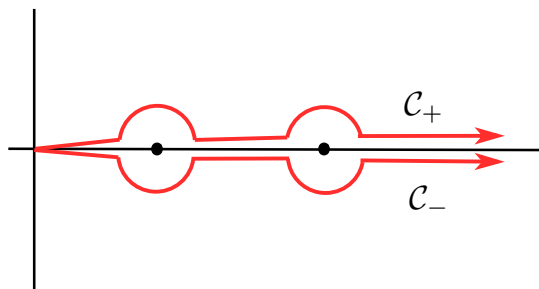
Figure 1. The paths C_{\pm} avoiding the singularities of the Borel transform from above (respectively, below).
