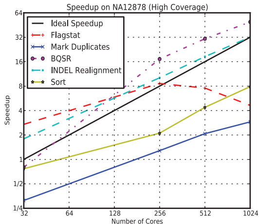
Figure 2: Speedup on NA12878
