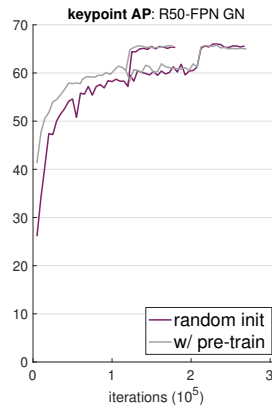
Figure 6. Keypoint detection on COCO using Mask R-CNN with R50-FPN and GN. We show keypoint AP on COCO val2017 . ImageNet pre-training has little benefit, and training from random initialization can quickly catch up without increasing training iterations. We only need to use 2\times and 3\times schedules, unlike the object detection case. The result is 65.6 vs. 65.5 (random initialization vs. pre-training) with 2\times schedules.
