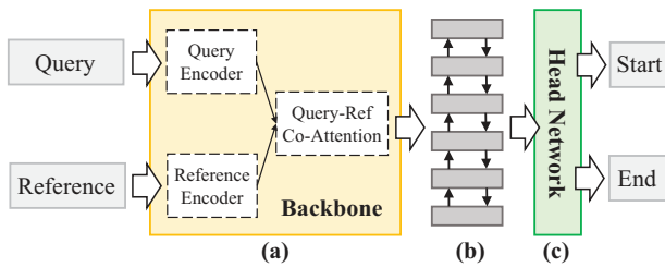
Figure 2: A typical bottom-up framework for QBVL. It always consists of a backbone (a) for query-ref interaction modeling and a head network (c) for boundaries prediction.
