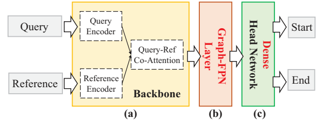
Figure 3: The architecture of GDP. It consists of a backbone (a), a Graph-FPN layer (b), and a dense head network (c).
