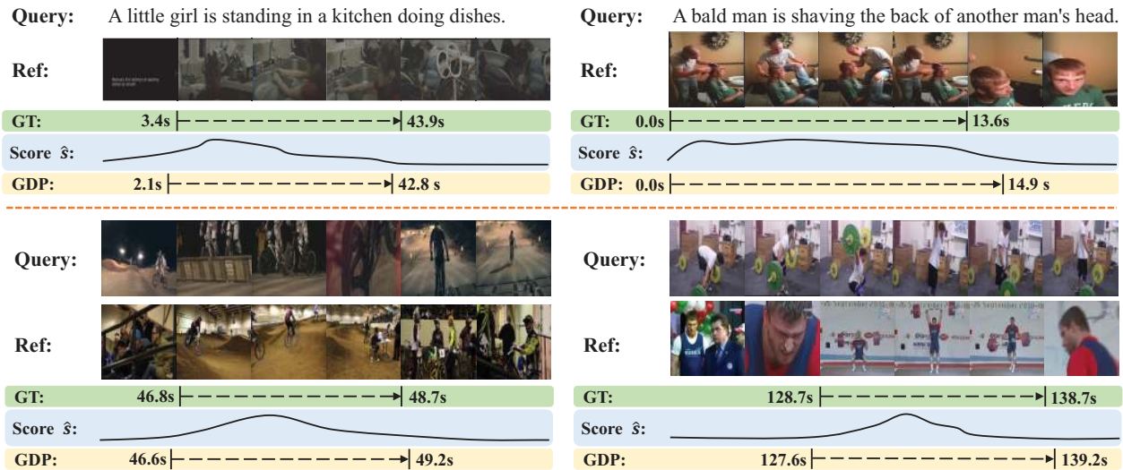
Figure 5: The qualitative results of GDP for NLVL on ActivityNet Captions (upper) and VRL on ActivityNet-VRL (below).
