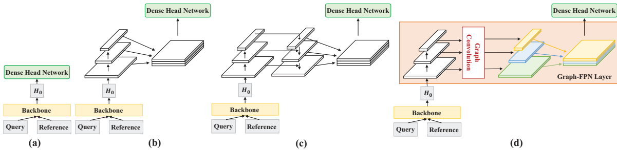
Figure 6: (a) Model A consists of a backbone and a dense head network. (b) Model B builds a pyramid hierarchy on top of backbone. (c) Model C uses FPN to combine two adjacent scale features. (d) Model D is the GDP with a Graph-FPN layer.
