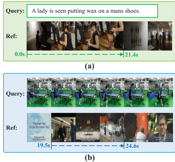
Figure 1: (a) Natural Language Video Localization: The query is a natural language; (b) Video Relocalization: The query is a video clip. Both tasks aim to localize a segment with start (0.0s/19.5s) and end (21.4s/24.6s) in the reference video (Ref) which semantically corresponds to the query.
