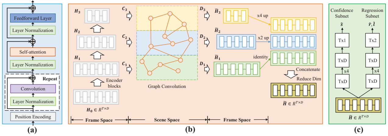
Figure 4: The details of each component of GDP. (a) The encoder block; (b) the Graph-FPN layer; (c) dense head network.
