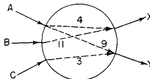
Fig. 7. A functional element with nonuniform propagation delays. The time at which output X must settle is either 4 esec after input A settles or 11 esec after input B settles, whichever is later.
