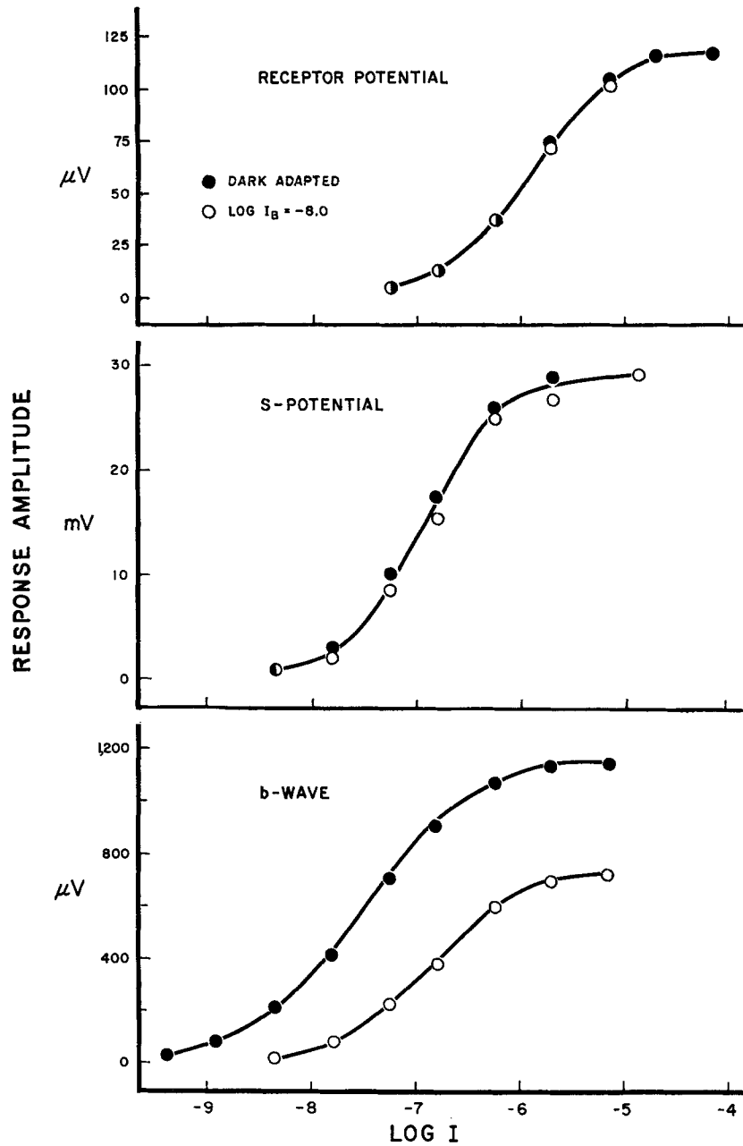
FIGURE 3. Intensity-response ( V -log- I ) curves for the receptor potential, S-potential, and b -wave recorded in the dark and in the presence of a dim adapting field ( \log I_B = -8 ). The V -log I curve of the b -wave is shifted by about 1 log unit to the right by this background field and its maximum amplitude is reduced. However the receptor potential and S-potential are not affected by this level of illumination. Data from representative single experiments.
