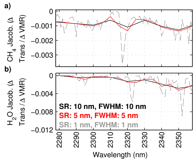
Fig. 16. (a) For the lowest layer of the atmospheric model (height up to 1.04 km), the CH 4 Jacobian calculated for AVIRISng (red) indicates improved sensitivity compared to the CH 4 Jacobian for AVIRIS (black). Even greater sensitivity can be achieved using a finer spectral resolution (SR) and FWHM (dashed grey). (b) H 2 O Jacobians calculated for the same three sensors.
