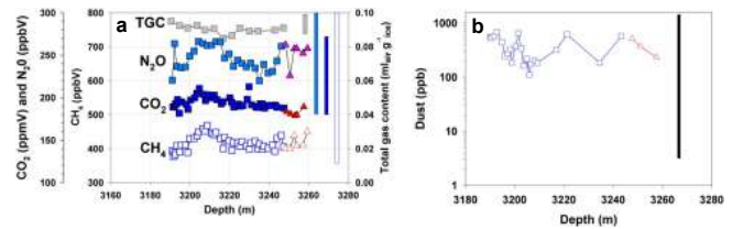
Figure 3. Gas and dust properties of the clean (squares) and dispersed (triangles) basal ice facies at EPICA Dome C: (a) total gas content ( \text{mL}_{\text{air ice}}^{-1} , grey), methane (ppbV, white), nitrous oxide (ppbV, light blue) and carbon dioxide (ppmV, dark blue) – vertical bars of equivalent shading cover the full concentration range observed for \text{CH}_4 , \text{CO}_2 , \text{N}_2\text{O} and total gas content during the preceding climatic cycles, (b) dust concentrations (ppb) – the black vertical bar covers the full concentration range during the previous climatic cycles.
