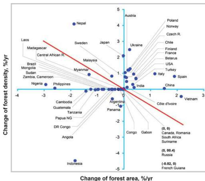
Fig. 5. A synoptic chart of changing forests during 1990–2005 in the 50 nations with the most growing stock reported in 2005. On the chart, the horizontal axis or longitude is the relative change of forest area ( a ), and the vertical axis or latitude is the relative change of growing stock density ( d ). Volume ( v ) was positive in nations above the diagonal line, a = -d , because growing stock was increasing.
