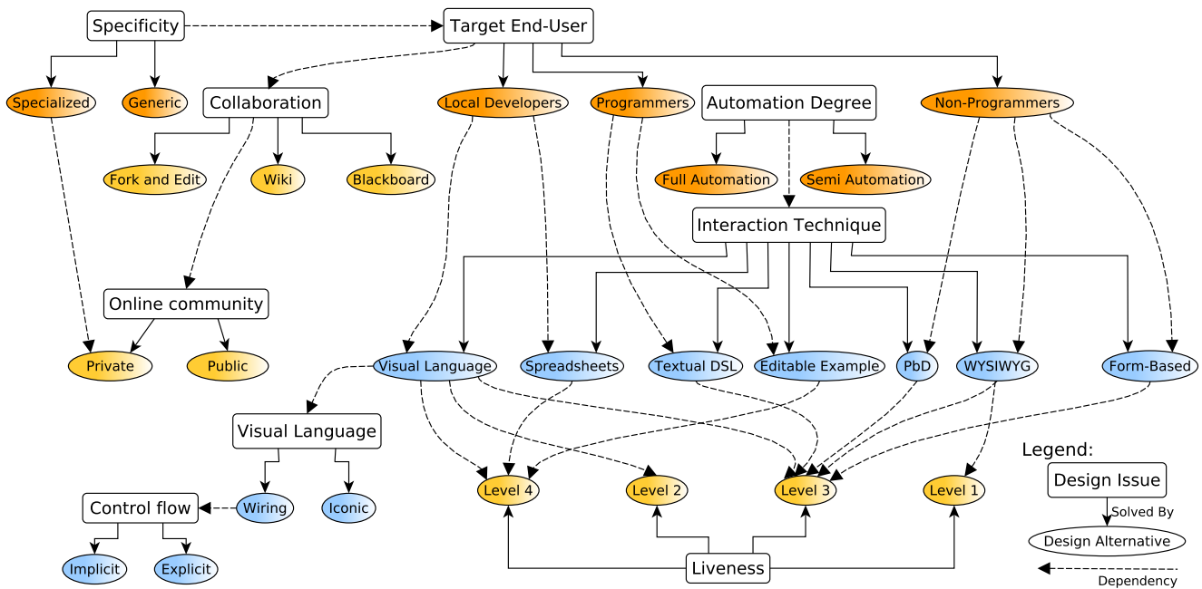
Figure 1. Mashup tool design space overview
