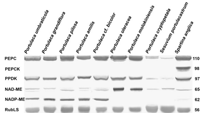
Fig. 3. Western blots for C 4 enzymes and Rubisco from total soluble proteins extracted from leaves of eight Portulaca species, the C 3 species Sesuvium portulacastrum , and the C 4 PEP-CK species Spartina anglica . Blots were probed with antibodies raised against PEPC, PPKK, NAD-ME, NADP-ME, PEP-CK, and Rubisco, respectively. Numbers on the left indicate molecular mass in kilodaltons. Subtle differences in blot intensity might occur due to differences in antigenicity between species.
