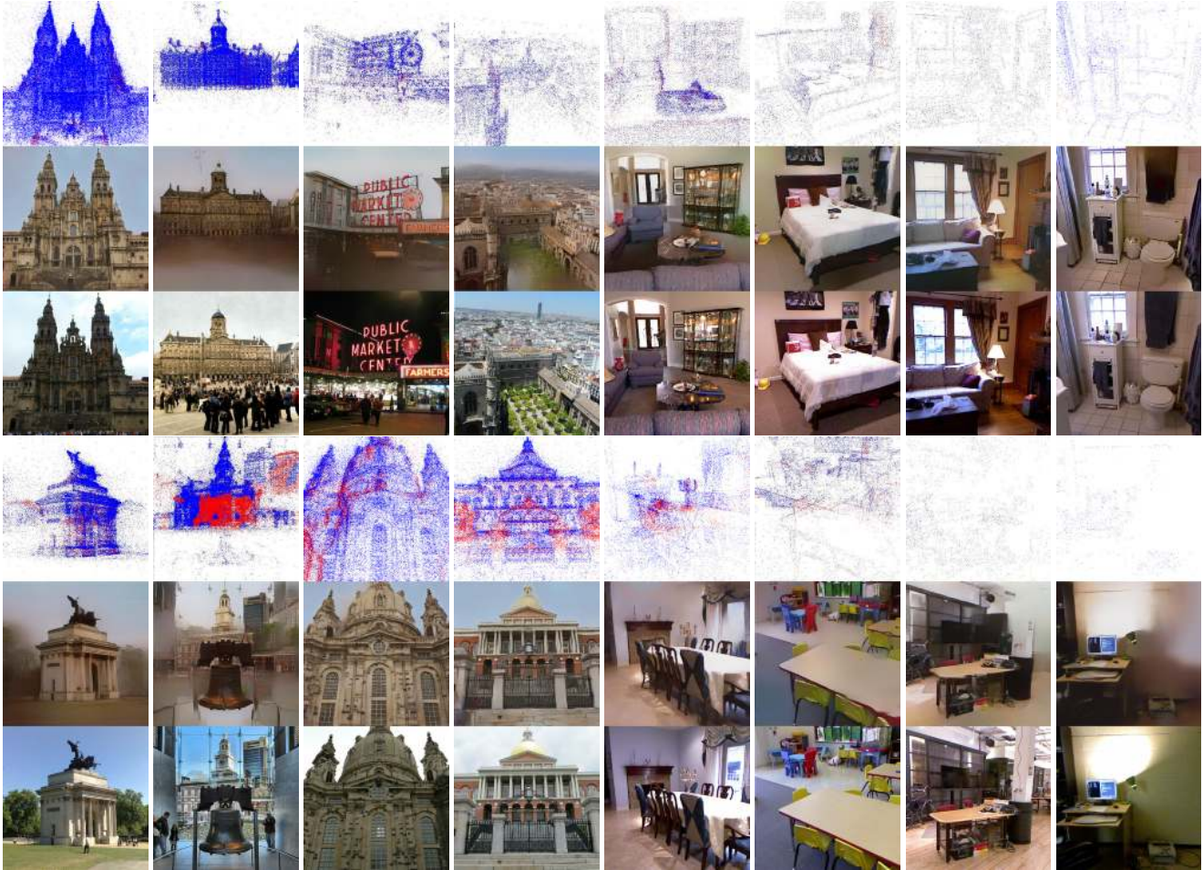
Figure 3: QUALITATIVE RESULTS: Each result is a 3 \times 1 set of square images, showing point clouds (with occluded points in red), image reconstruction and original. The first four columns (top and bottom) show results from the MegaDepth dataset (internet scenes) and the last four columns (top and bottom) show results from indoor NYU scenes. Sparsity: Our network handles a large variety in input sparsity (density decreases from left to right). In addition, perspective projection accentuates the spatially-varying density differences, and the MegaDepth outdoor scenes have concentrated points in the input whereas NYU indoor scenes have far samples. Further, the input points are non-homogeneous, with large holes which our method gracefully fills in. Visual effects: For the first four columns (MD scenes) our results give the pleasing effect of uniform illumination (see top of first column). Since our method relies on SfM, moving objects are not recovered. Scene diversity: The fourth column is an aerial photograph, an unusual category that is still recovered well. For the last four columns (NYU scenes), despite lower sparsity, we can recover textures in common household scenes such as bathrooms, classrooms and bedrooms. The variety shows that our method does not learn object categories and works on any scene. Visibility: All scenes benefit from visibility prediction using VISIBNET which for example was crucial for the bell example (lower 2 nd column).
