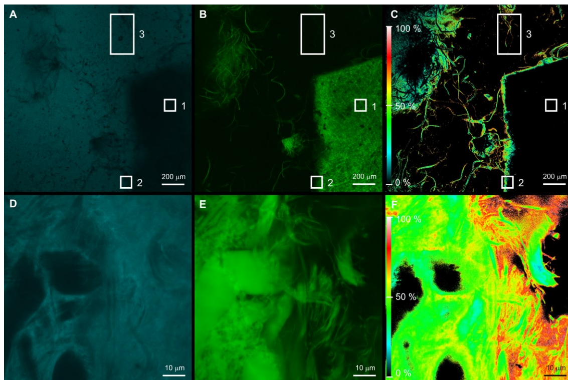
Figure 5. FRET/LSCM false-color images for PE-C30+FLNFCp: (A) C30 fluorescence (donor filter set) at 5x magnification; (B) FLNFC fluorescence (acceptor filter set) at 5x; (C) energy-transfer-efficiency map calculated according to the N_{FRET} algorithm at 5x ( N_{FRET} = 0.010 ); (D) C30 fluorescence at 100x; (E) FLNFC fluorescence at 100x; (F) energy-transfer-efficiency map at 100x.
