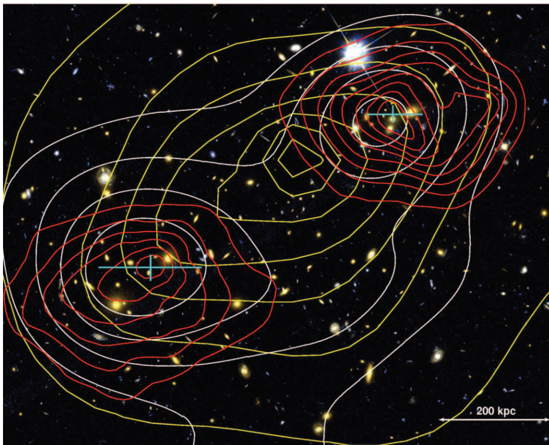
FIG. 4.—F555W-F814W color composite of the cluster MACS J0025.4–1222. North is up and east is to the left. The field is 2.5' \times 2.0' , which corresponds to 1000 \times 800 \text{ kpc}^2 at the redshift of the cluster. Overlaid in red contours is the surface mass density \kappa from the combined weak- and strong-lensing mass reconstruction. The contour levels are linearly spaced with \Delta\kappa = 0.1 , starting at \kappa = 0.5 , for a fiducial source at a redshift of z_s \rightarrow \infty . The X-ray brightness contours (also linearly spaced) are overlaid in yellow, and the I -band light is overlaid in white. The measured peak position and error bars for the total mass are given as a cyan cross (see Table 2).
