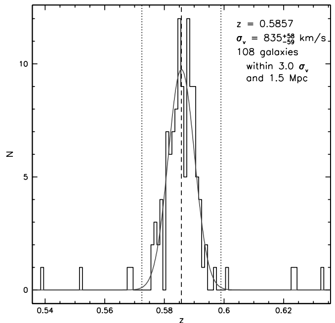
FIG. 1.—Histogram of the redshift distribution around the cluster redshift. Only galaxies within projected 1.5 Mpc are shown. The dashed line indicates the cluster redshift, the dotted lines the \pm 3 \sigma_{\text{CI}} limits used to calculate the cluster redshift and velocity dispersion. The Gaussian curve overplotted in gray illustrates the measured velocity dispersion. [See the electronic edition of the Journal for a color version of this figure.]
