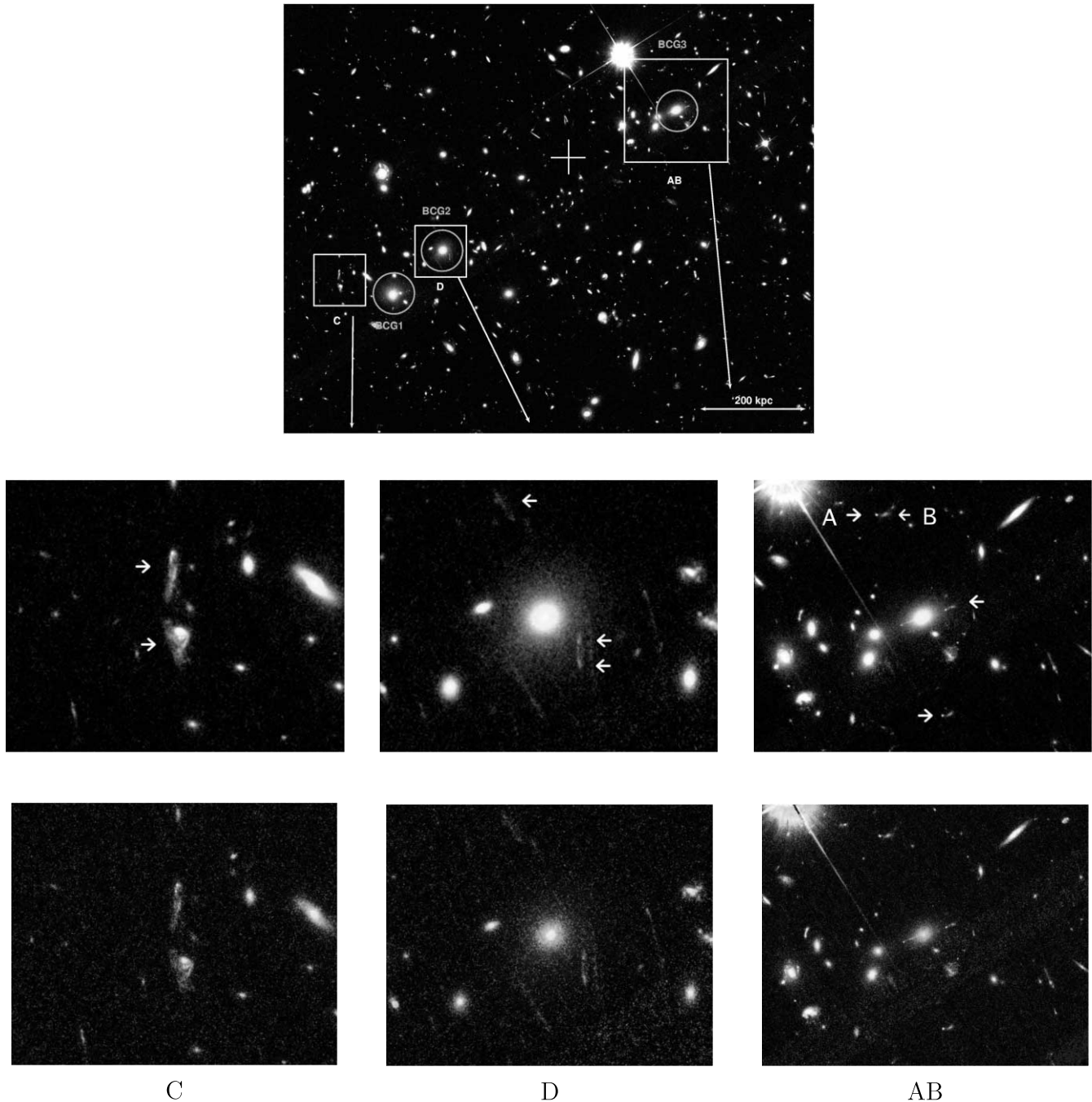
FIG. 2.— Top : F555W-F814W color composite of the cluster MACS J0025.4–1222. North is up and east is to the left. The field is 2.5' \times 2.0' . Also shown are 15'' \times 15'' cutouts (indicated in top panel) of C and D and 30'' \times 30'' of the multiply imaged systems AB from the F555W-F814W (middle row) and F450W-F555W-F814W (bottom row) color composite. The three BCGs are marked with circles, the gas peak position with a cross (with its size indicating the measured uncertainty; see § 5). [See the electronic edition of the Journal for a color version of this figure.]
