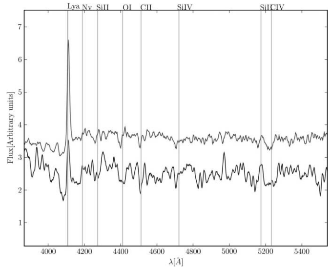
FIG. 3.—LRIS spectrum of the images A and B (a single slit was placed over both images). Lines redshifted to z = 2.38 are marked. Overplotted (and offset for clarity) in gray (top) is the composite Lyman break galaxy spectrum from Shapley et al. (2003). The emission line is significantly detected ( 6\sigma ); no other significant features are seen in the spectrum. [See the electronic edition of the Journal for a color version of this figure.]
