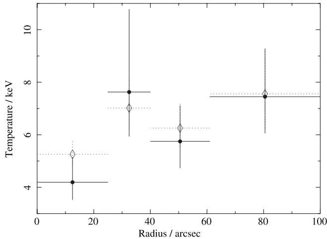
FIG. 5.—Temperature profiles of the X-ray gas. Open diamonds show the projected values, filled circles the deprojected values (assuming spherical symmetry and using a project model to account for geometric effects). Error bars are 1\sigma . [See the electronic edition of the Journal for a color version of this figure.]
