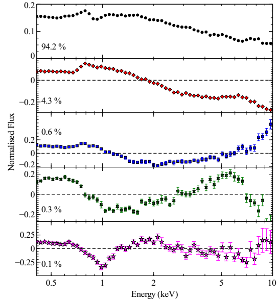
Figure 15. Principal component spectra found in NGC 4051, ordered from top to bottom by the fraction of variability in each component. PCs one, two, three and four correspond to one, two and four and three from MCG-06-30-15, and the additional component 5 appears to be attributable to a variable absorption feature.
