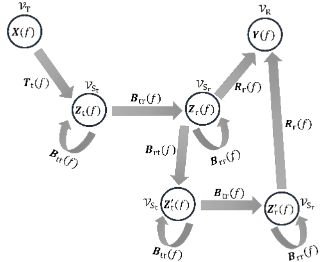
Fig. 12. Schematic diagram for the vector signal flow representing the PG for room-to-room scenario, assuming there is 1 time propagation from \mathcal{R}_r to \mathcal{R}_t
