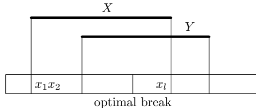
Figure 1: Illustration of Lemma 4
